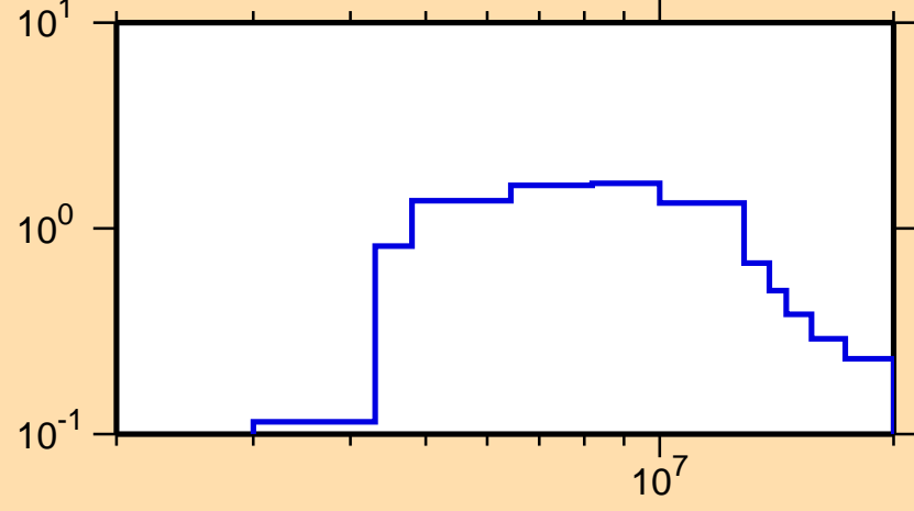
\sigma vs. E for ^{84}\text{Kr}(n,n\text{cont.})
