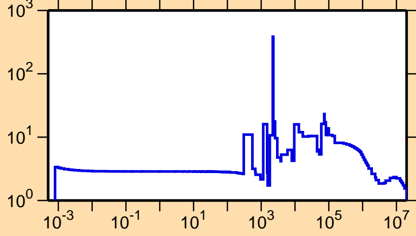
\sigma vs. E for ^{84}\text{Kr}(n,\text{el.})
