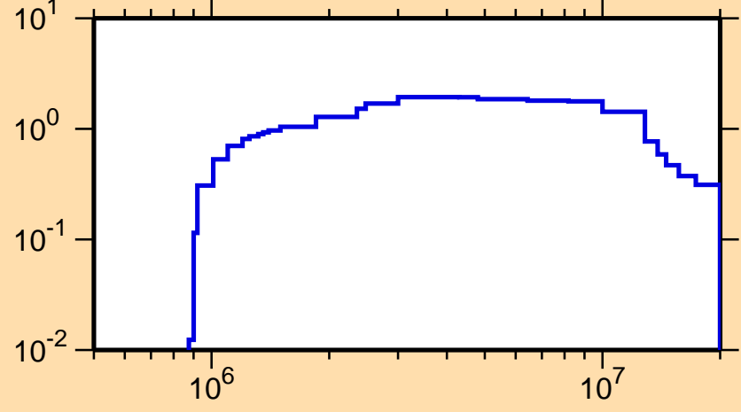
\sigma vs. E for ^{84}\text{Kr}(n,\text{inel.})
