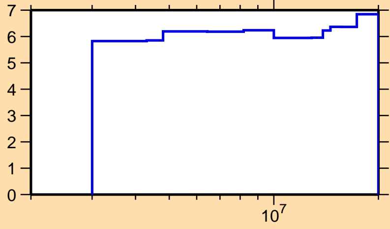
\Delta\sigma/\sigma vs. E for ^{84}\text{Kr}(n,n\text{onel.})
