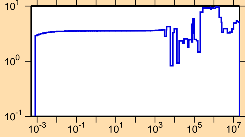
\Delta\sigma/\sigma vs. E for ^{82}\text{Se}(n,\text{tot.})
