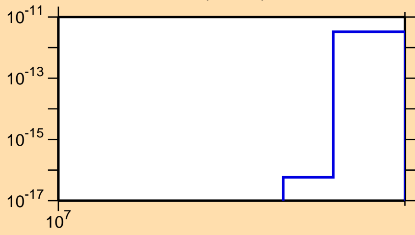
\sigma vs. E for ^{75}\text{Se} (mt 45)
