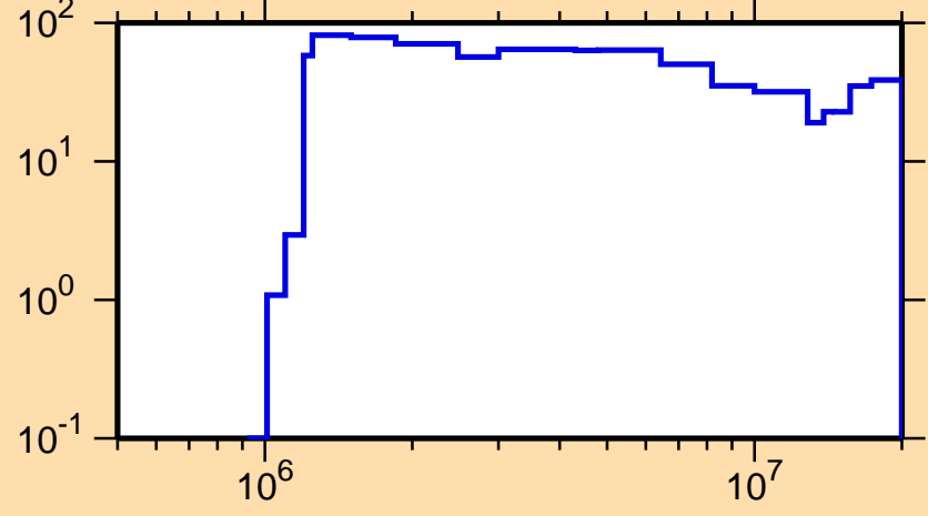
\Delta\sigma/\sigma vs. E for ^{74}\text{Se}(n,p)
