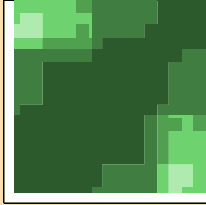
\sigma vs. E for ^{74}\text{Se}(n,\text{inel.})
