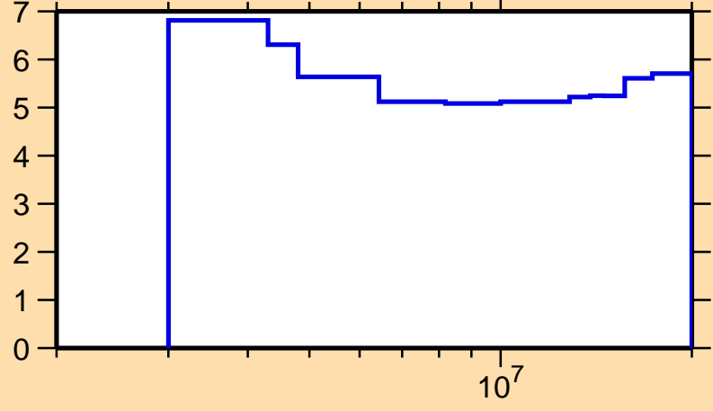
\Delta\sigma/\sigma vs. E for ^{74}\text{Se}(n,n\text{onel.})
