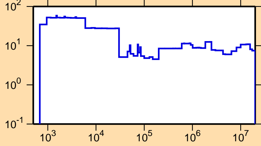
\Delta\sigma/\sigma vs. E for ^{74}\text{As}(n,\text{el.})
