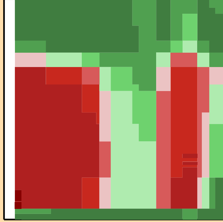
\Delta\sigma/\sigma vs. E for ^{74}\text{As}(n,n\text{cont.})
