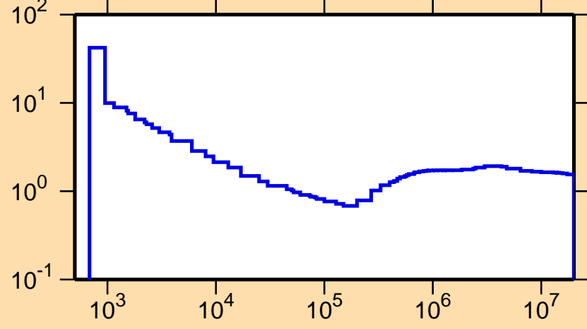
\sigma vs. E for ^{74}\text{As}(n,\text{nonel.})
