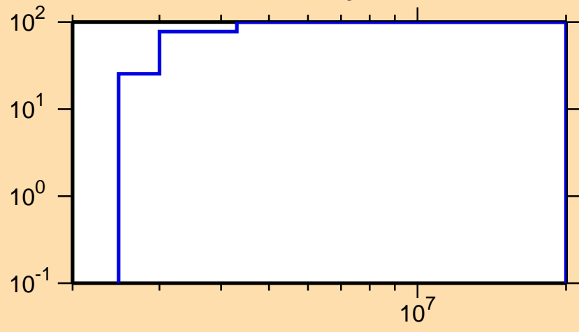
\Delta\sigma/\sigma vs. E for ^{59}\text{Ni}(n,n_{13})
