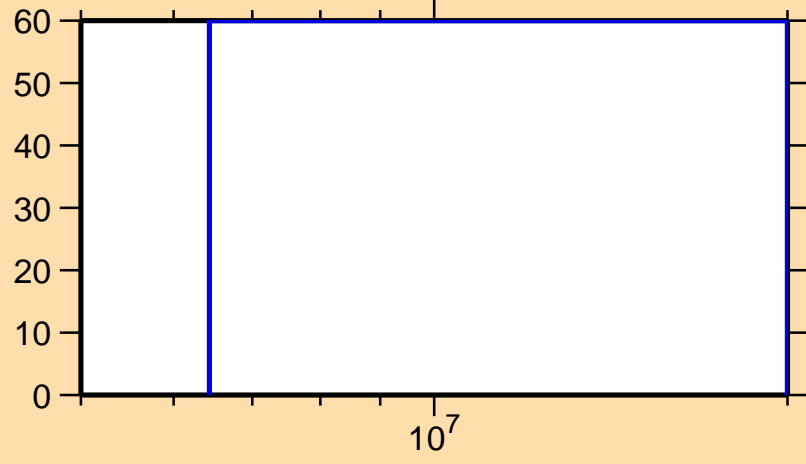
\Delta\sigma/\sigma vs. E for ^{59}\text{Ni}(n,n_0)
