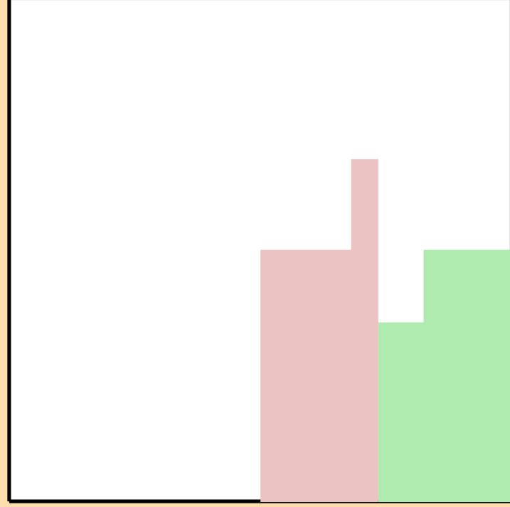
\Delta\sigma/\sigma vs. E for ^{59}\text{Ni}(n,np)
