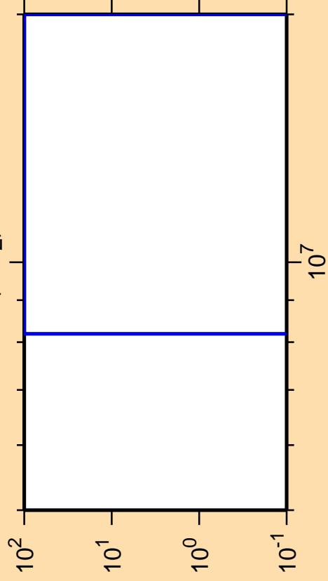
\Delta\sigma/\sigma vs. E for ^{59}\text{Ni}(n,n_2)
