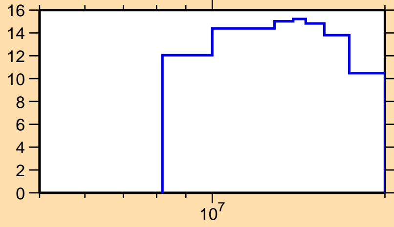
\Delta\sigma/\sigma vs. E for ^{59}\text{Ni}(n,el.)
