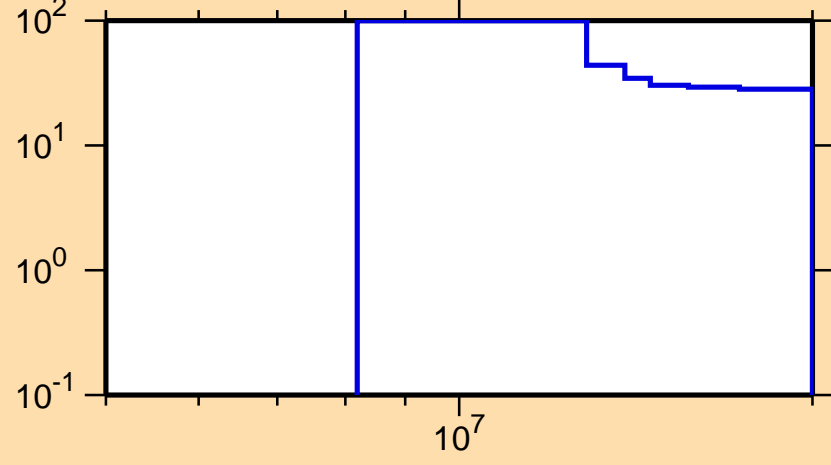
\Delta\sigma/\sigma vs. E for ^{59}\text{Ni}(n,np)
