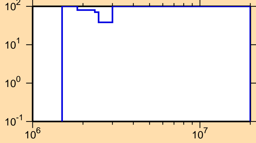
\Delta\sigma/\sigma vs. E for ^{59}\text{Ni}(n,n_{12})
