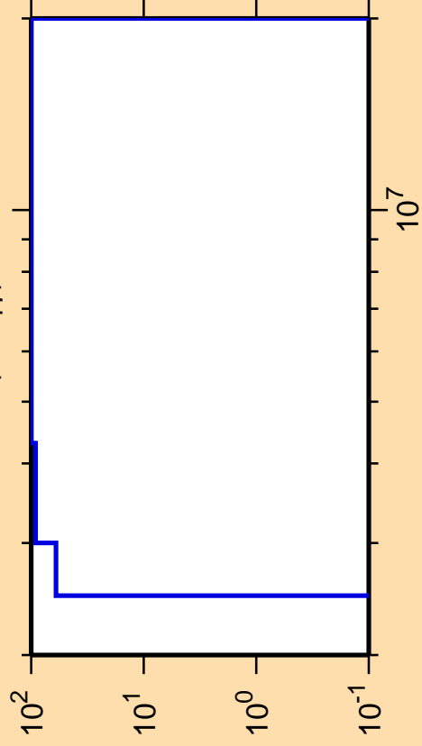
\Delta\sigma/\sigma vs. E for ^{59}\text{Ni}(n,n_{17})
