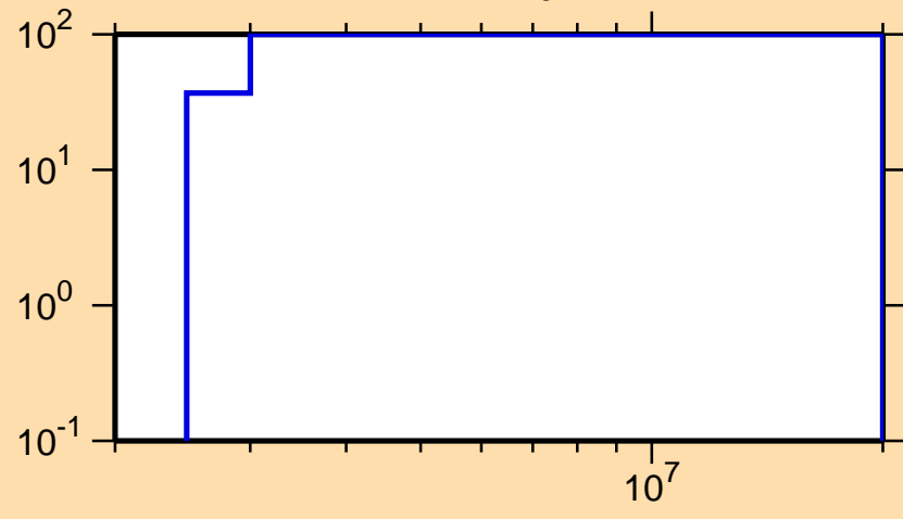
\Delta\sigma/\sigma vs. E for ^{59}\text{Ni}(n,n_{10})
