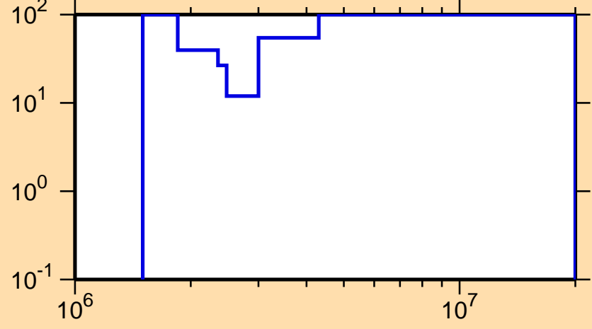
\Delta\sigma/\sigma vs. E for ^{59}\text{Ni}(n,n_9)
