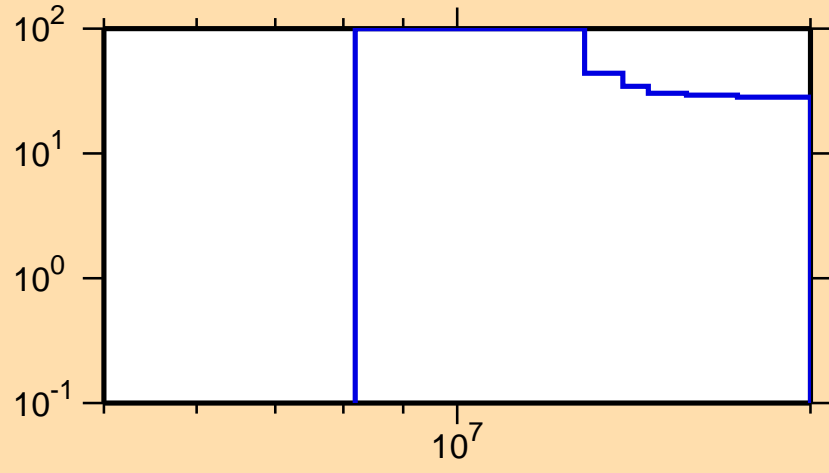
\Delta\sigma/\sigma vs. E for ^{59}\text{Ni}(n,np)
