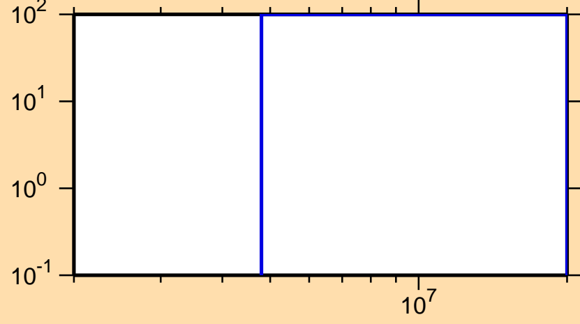
\Delta\sigma/\sigma vs. E for ^{59}\text{Ni}(n,n\alpha)
