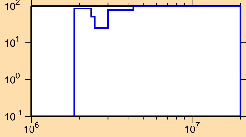
\Delta\sigma/\sigma vs. E for ^{59}\text{Ni}(n,n_{13})
