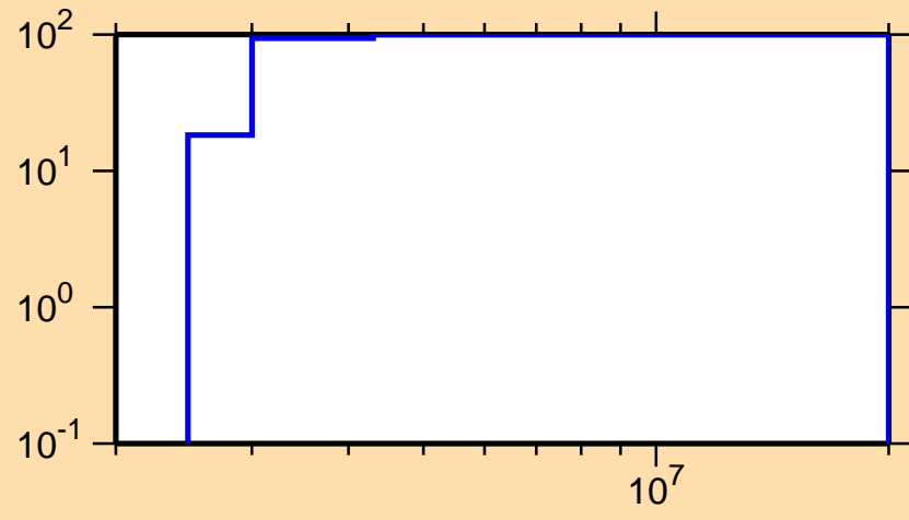
\Delta\sigma/\sigma vs. E for ^{59}\text{Ni}(n,n_2)
