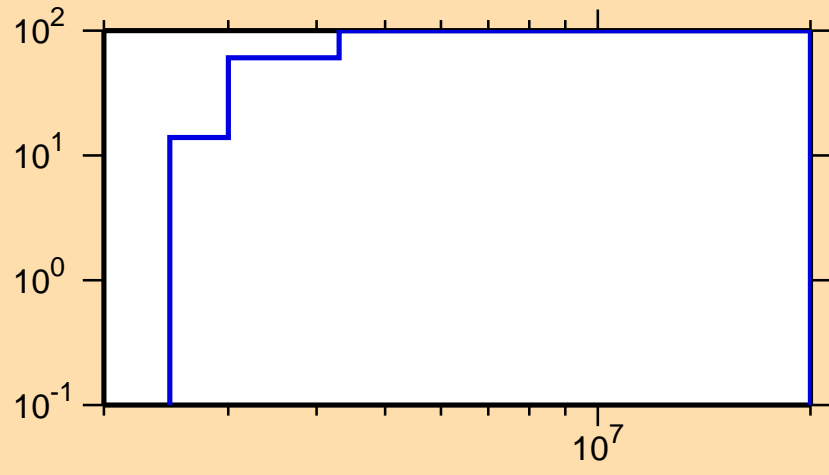
\Delta\sigma/\sigma vs. E for ^{59}\text{Ni}(n,n_3)
