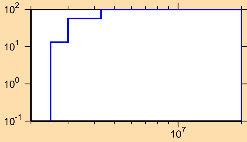
\Delta\sigma/\sigma vs. E for ^{59}\text{Ni}(n,n_4)
