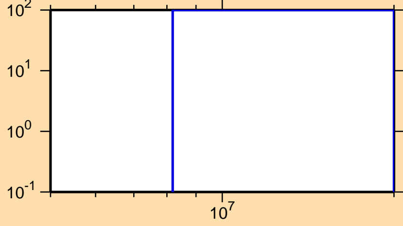
\Delta\sigma/\sigma vs. E for ^{59}\text{Ni}(n,n_{17})
