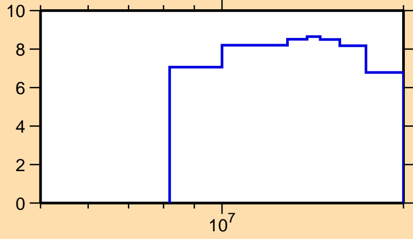
\Delta\sigma/\sigma vs. E for ^{59}\text{Ni}(n,tot.)
