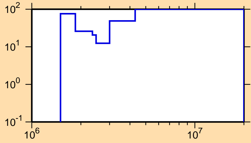
\Delta\sigma/\sigma vs. E for ^{59}\text{Ni}(n,n_7)
