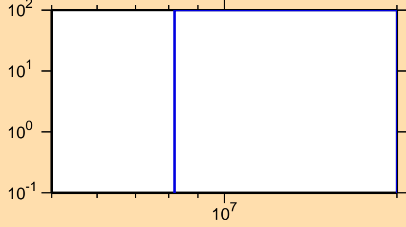
\Delta\sigma/\sigma vs. E for ^{59}\text{Ni}(n,t)
