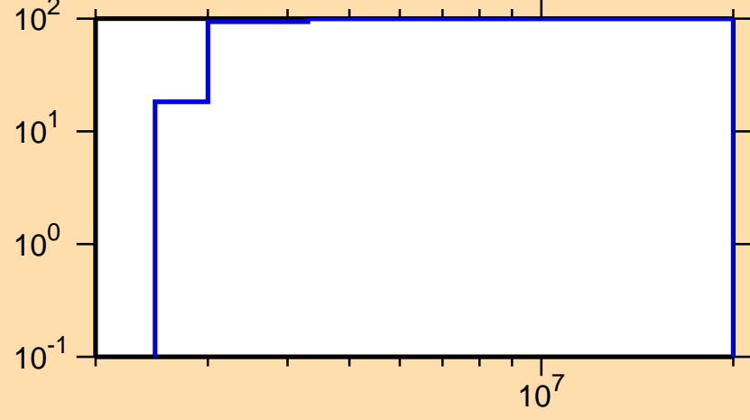
\Delta\sigma/\sigma vs. E for ^{59}\text{Ni}(n,n_2)
