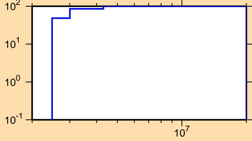
\Delta\sigma/\sigma vs. E for ^{59}\text{Ni}(n,n_{14})
