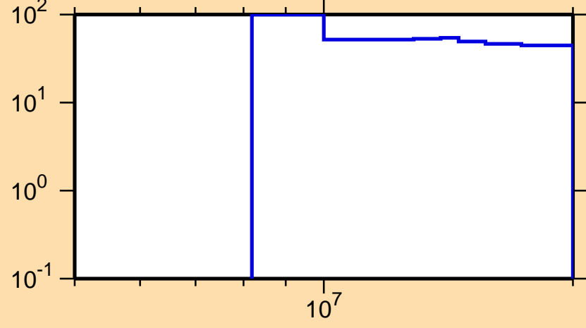
\Delta\sigma/\sigma vs. E for ^{59}\text{Ni}(n,2n)
