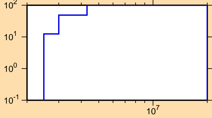
\Delta\sigma/\sigma vs. E for ^{59}\text{Ni}(n,n_7)
