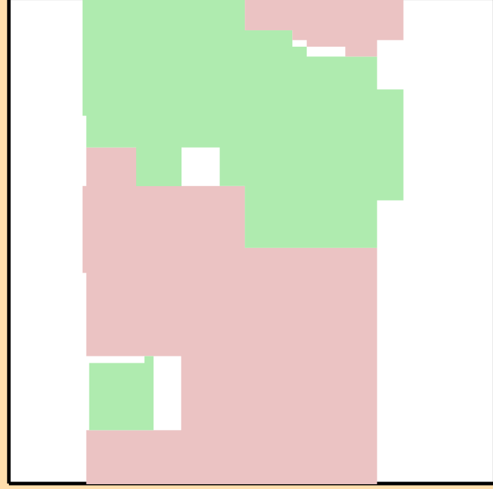
\Delta\sigma/\sigma vs. E for ^{59}\text{Ni}(n,n_3)
