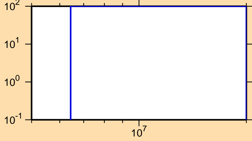
\Delta\sigma/\sigma vs. E for ^{59}\text{Ni}(n,\text{He3})
