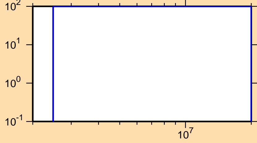
\Delta\sigma/\sigma vs. E for ^{59}\text{Ni}(n,n_{18})
