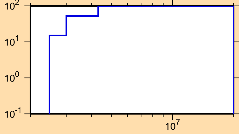
\Delta\sigma/\sigma vs. E for ^{59}\text{Ni}(n,n_6)
