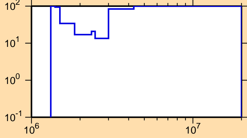
\Delta\sigma/\sigma vs. E for ^{59}\text{Ni}(n,n_5)
