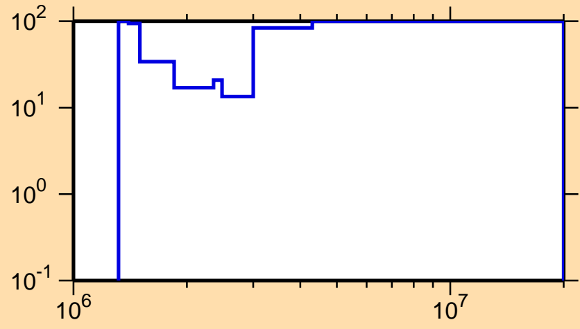
\Delta\sigma/\sigma vs. E for ^{59}\text{Ni}(n,n_5)
