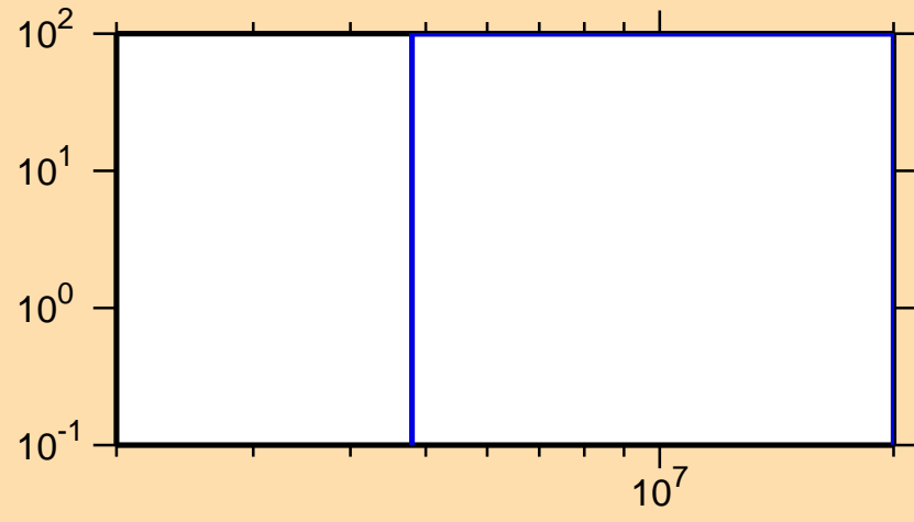
\Delta\sigma/\sigma vs. E for ^{59}\text{Ni}(n,n\alpha)
