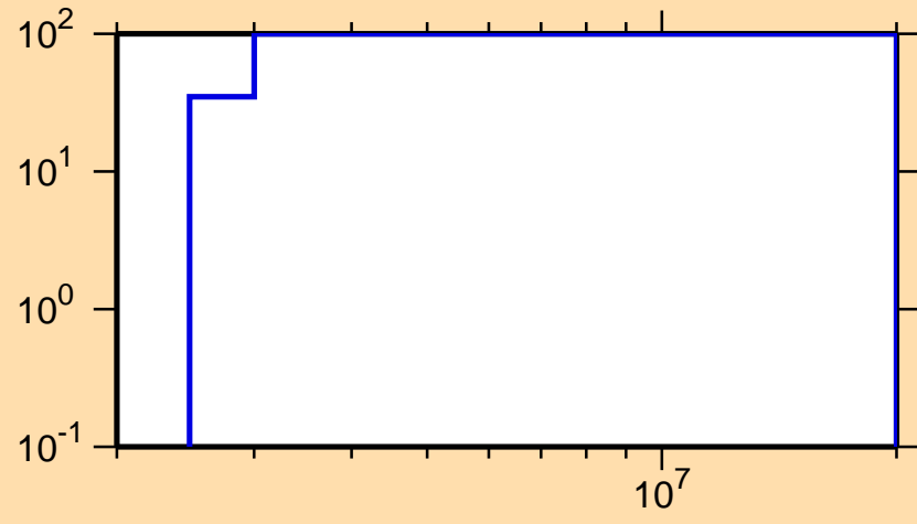
\Delta\sigma/\sigma vs. E for ^{59}\text{Ni}(n,n_8)
