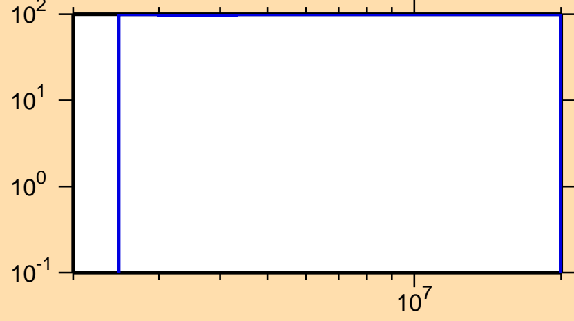
\Delta\sigma/\sigma vs. E for ^{59}\text{Ni}(n,n_{19})
