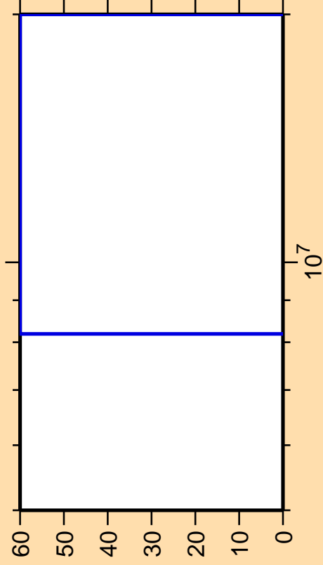
\Delta\sigma/\sigma vs. E for ^{59}\text{Ni}(n,n_7)
