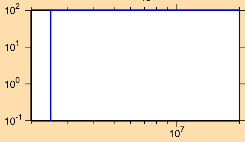
\Delta\sigma/\sigma vs. E for ^{59}\text{Ni}(n,n_{16})
