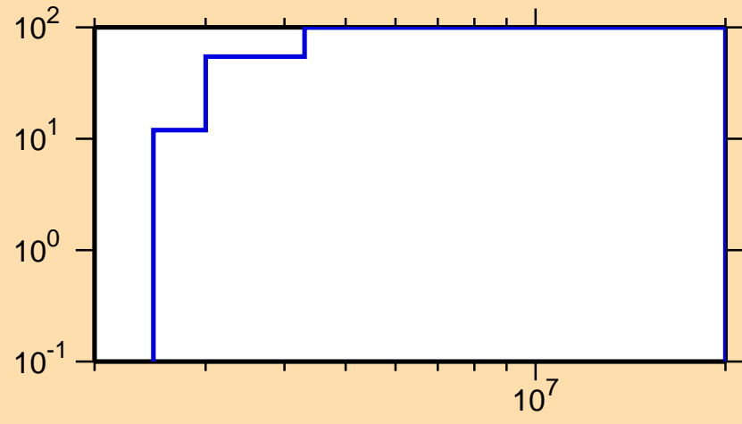
\Delta\sigma/\sigma vs. E for ^{59}\text{Ni}(n,n_9)
