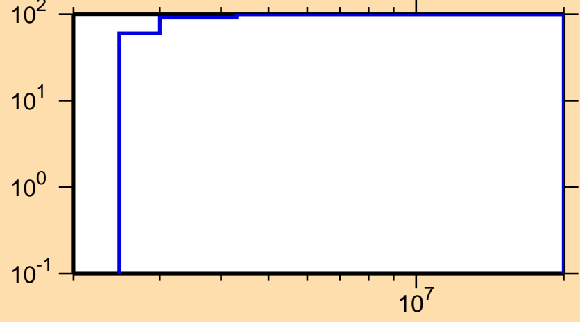
\Delta\sigma/\sigma vs. E for ^{59}\text{Ni}(n,n_{17})
