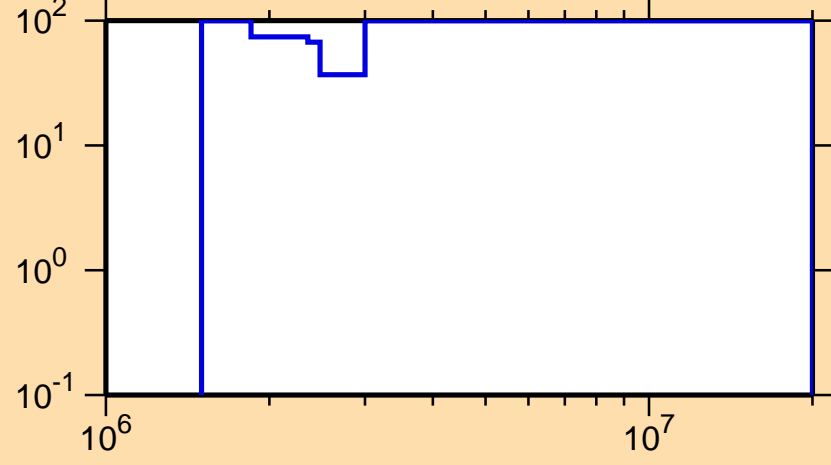
\Delta\sigma/\sigma vs. E for ^{59}\text{Ni}(n,n_{10})
