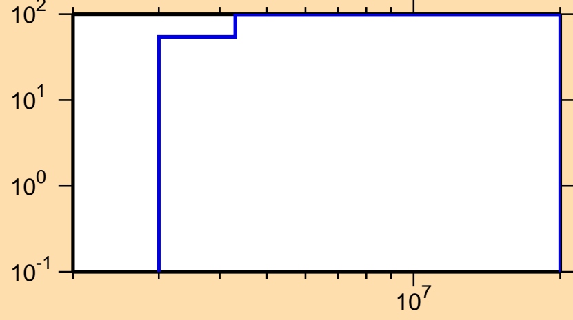
\Delta\sigma/\sigma vs. E for ^{59}\text{Ni}(n,n_g)
