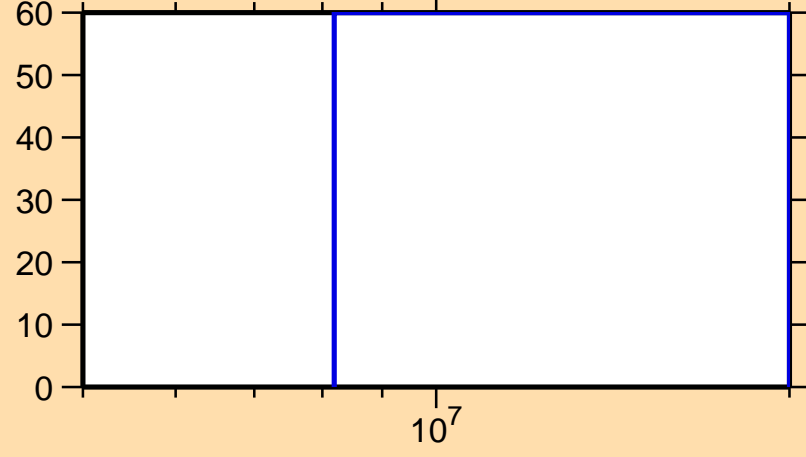
\Delta\sigma/\sigma vs. E for ^{59}\text{Ni}(n,n_6)
