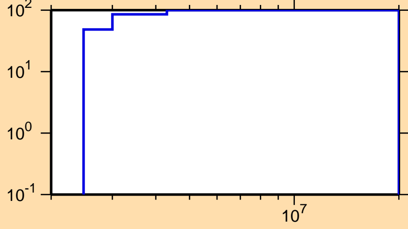
\Delta\sigma/\sigma vs. E for ^{59}\text{Ni}(n,n_{14})
