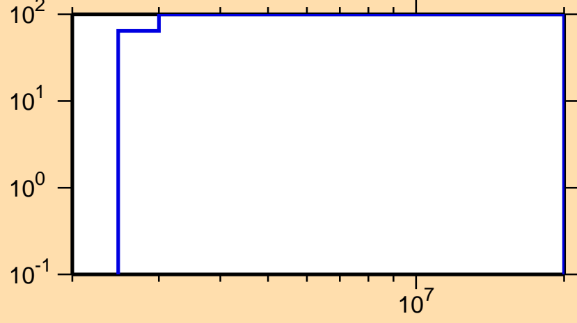
\Delta\sigma/\sigma vs. E for ^{59}\text{Ni}(n,n_{15})
