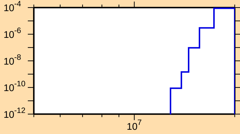
\sigma vs. E for ^{69}\text{Ga}(n,\text{He3})
