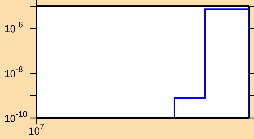
\sigma vs. E for ^{69}\text{Ga}(n,\text{nt})
