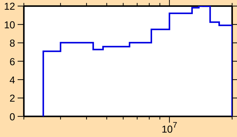
\Delta\sigma/\sigma vs. E for ^{69}\text{Ga}(\text{n},\text{el.})
