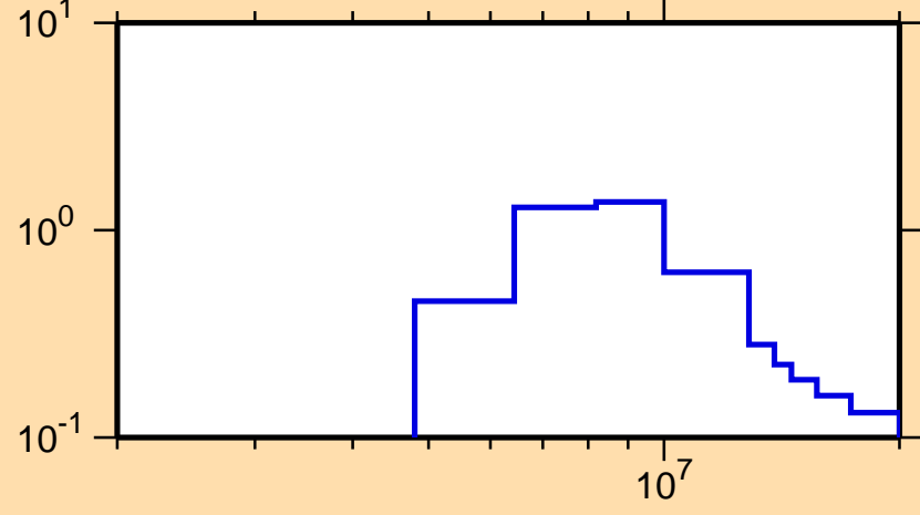
\sigma vs. E for ^{66}\text{Ni}(n,n\text{cont.})
