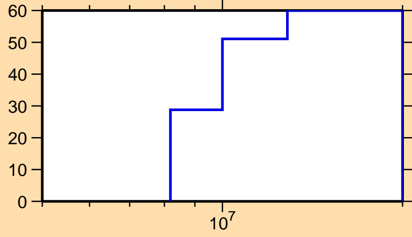
\Delta\sigma/\sigma vs. E for ^{66}\text{Ni}(n,ncont.)
