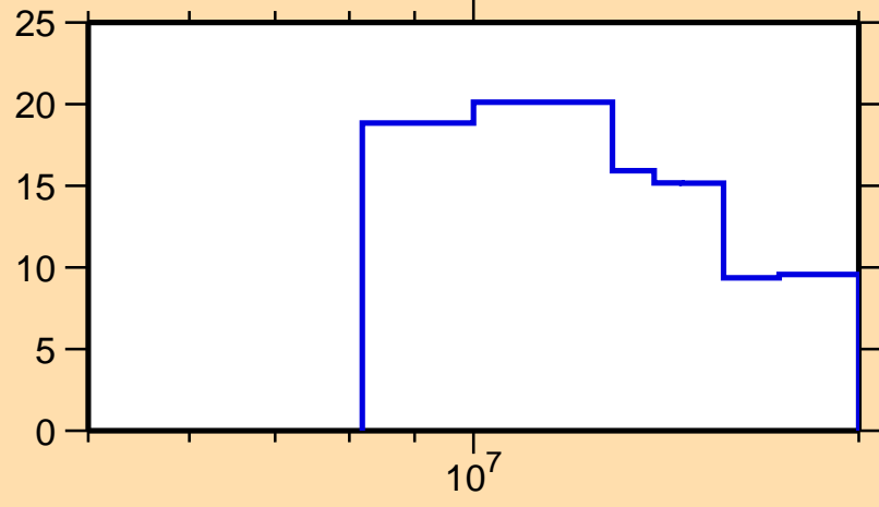
\Delta\sigma/\sigma vs. E for ^{66}\text{Ni}(n,el.)
