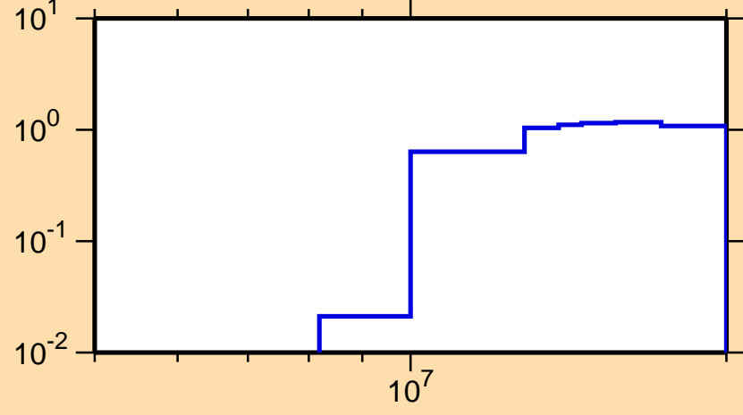
\sigma vs. E for ^{67}\text{Cu}(n,2n)
