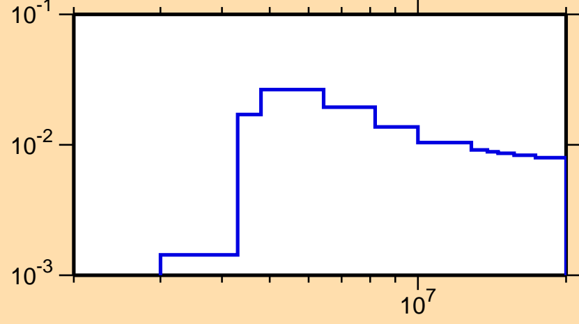
\sigma vs. E for ^{56}\text{Ni}(n,n_2)
