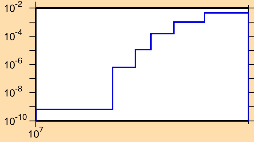
\sigma vs. E for ^{56}\text{Ni}(n,pd)
