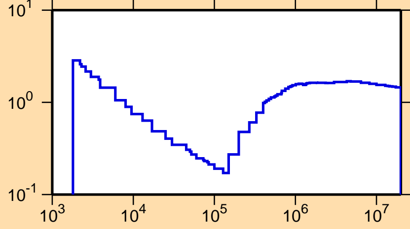
\sigma vs. E for ^{64}\text{Cu}(n,\text{nonel.})
