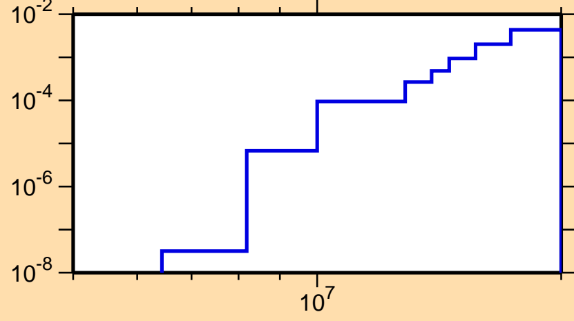
\sigma vs. E for ^{64}\text{Cu}(n,t)
