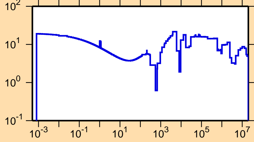
\Delta\sigma/\sigma vs. E for ^{63}\text{Ni}(n,\text{tot.})
