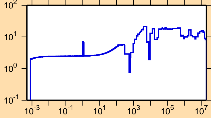
\Delta\sigma/\sigma vs. E for ^{63}\text{Ni}(n,\text{el.})
