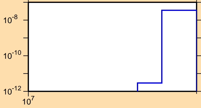
\sigma vs. E for ^{63}\text{Ni}(n,\text{He}3)
