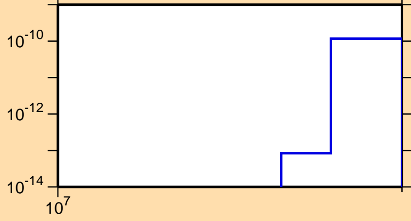
\sigma vs. E for ^{62}\text{Co}(n,p\alpha)
