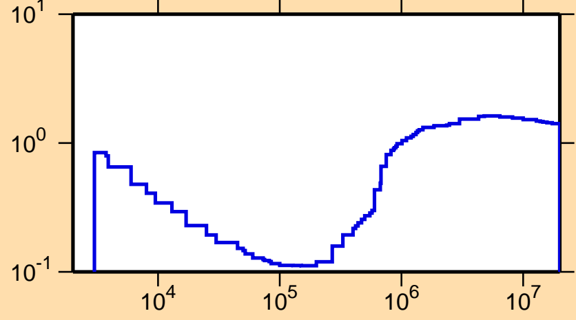
\sigma vs. E for ^{62}\text{Co}(n,\text{nonel.})
