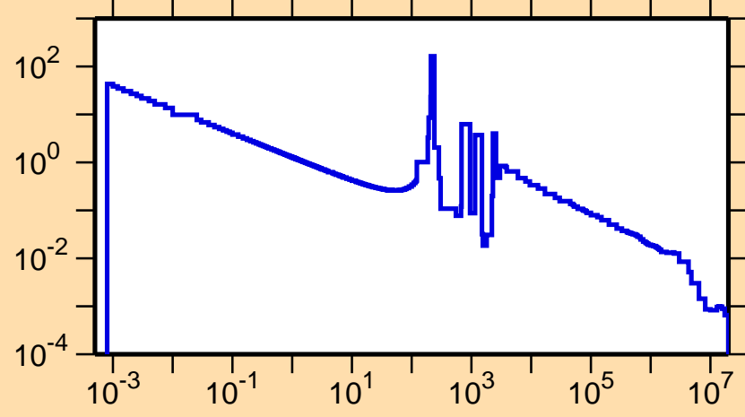
\sigma vs. E for ^{62}\text{Co}(n,\gamma)
