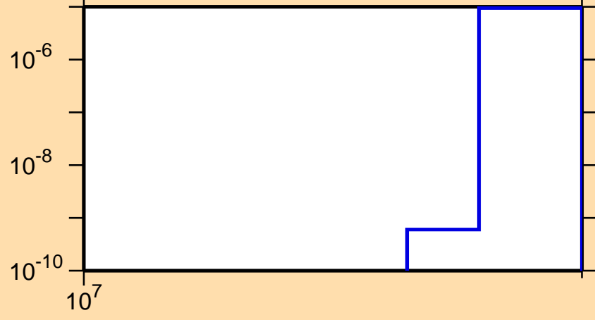
\sigma vs. E for ^{62}\text{Co}(n,nt)
