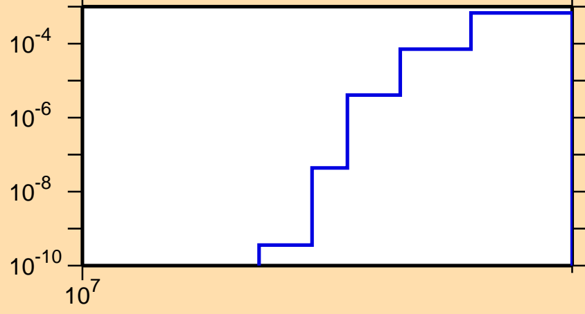
\sigma vs. E for ^{62}\text{Ni}(n,t)
