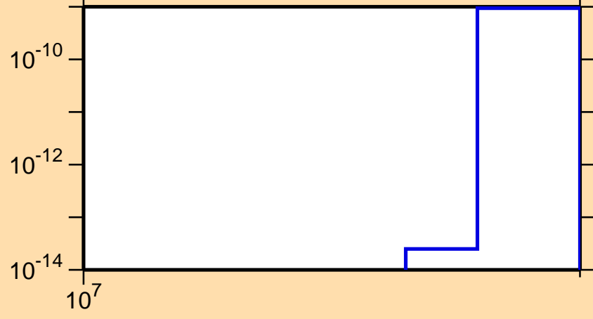
\sigma vs. E for ^{62}\text{Ni}(n,p\alpha)
