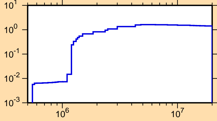
\sigma vs. E for ^{62}\text{Ni}(n,\text{nonel.})
