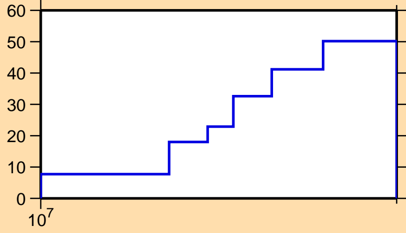
\Delta\sigma/\sigma vs. E for ^{58}\text{Fe}(n,inel.)
