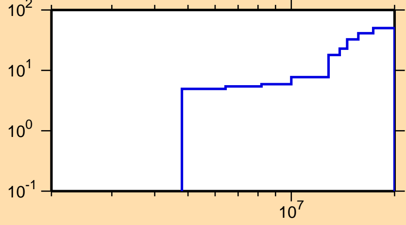
\Delta\sigma/\sigma vs. E for ^{58}\text{Fe}(n,\text{inel.})
