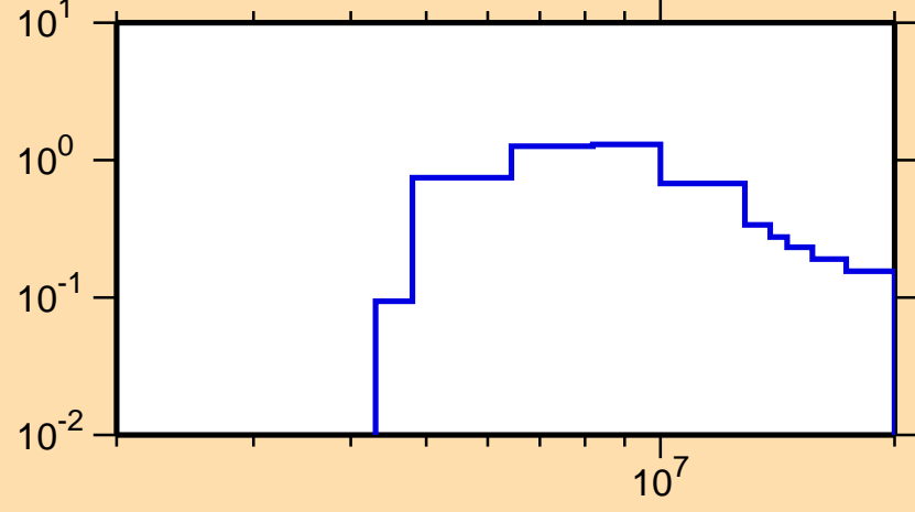
\sigma vs. E for ^{60}\text{Fe}(n,n\text{cont.})
