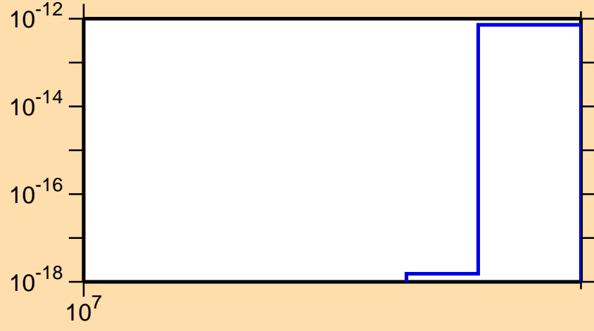
\sigma vs. E for ^{60}\text{Fe}(n,2n\alpha)
