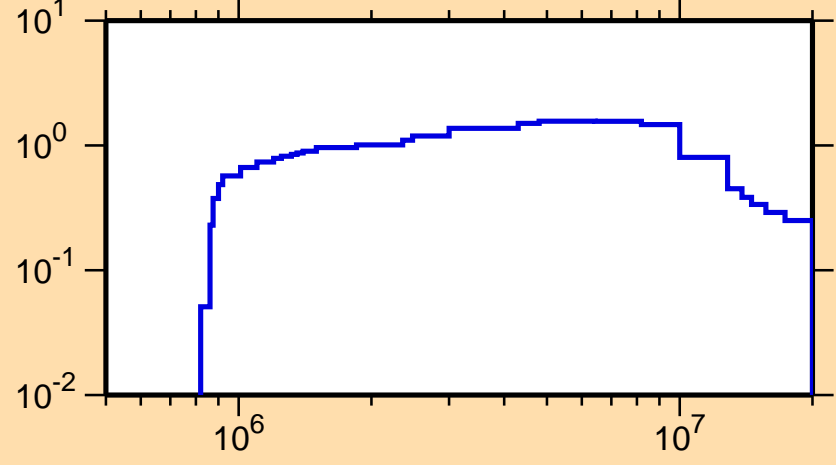
\sigma vs. E for ^{60}\text{Fe}(n,\text{inel.})
