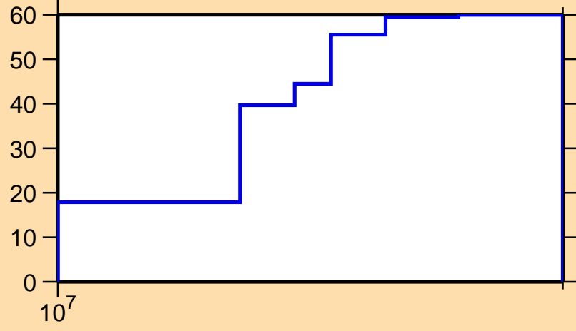
\Delta\sigma/\sigma vs. E for ^{57}\text{Fe}(n,inel.)
