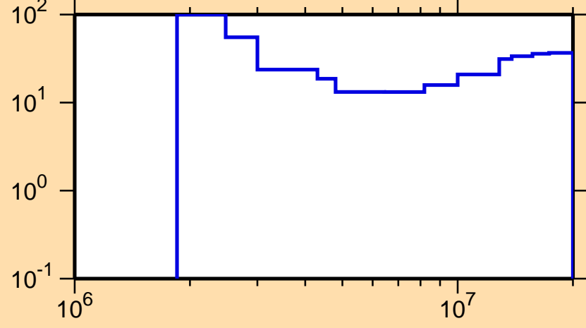
\Delta\sigma/\sigma vs. E for ^{54}\text{Mn}(n,n\text{cont.})
