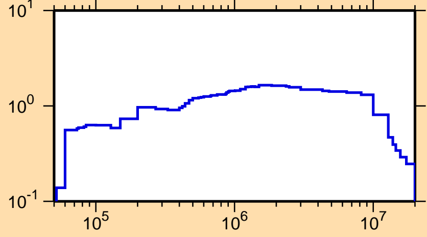
\sigma vs. E for ^{54}\text{Mn}(n,\text{inel.})
