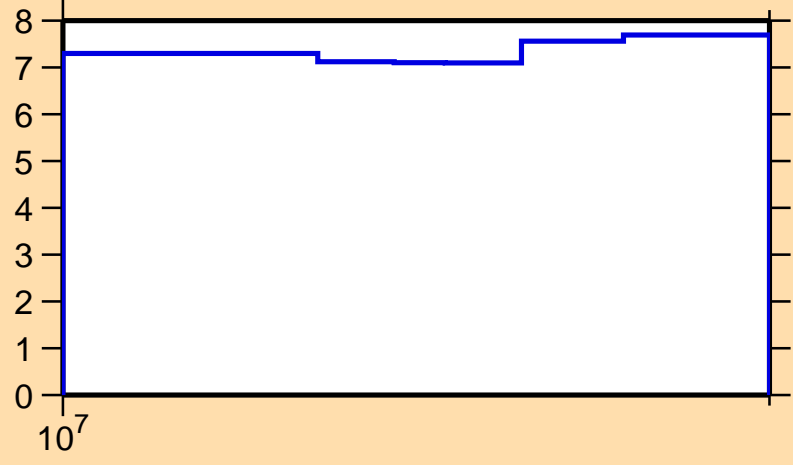
\Delta\sigma/\sigma vs. E for ^{49}\text{V}(n,\text{nonel.})
