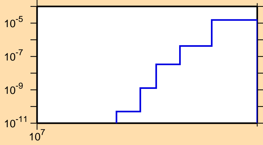
\sigma vs. E for ^{49}\text{V}(n,\text{He3})
