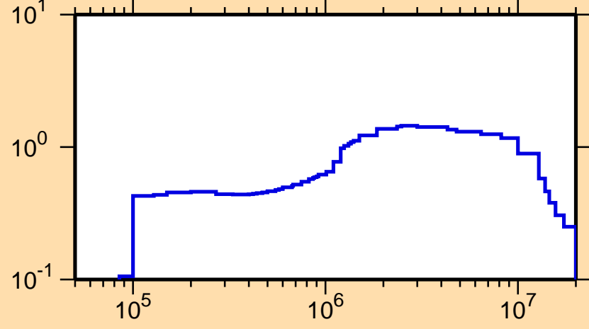
\sigma vs. E for ^{49}\text{V}(n,\text{inel.})
