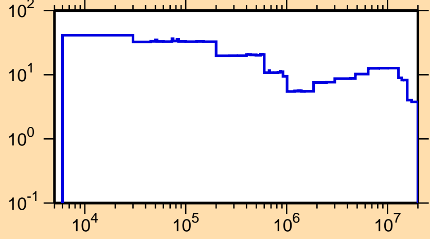
\Delta\sigma/\sigma vs. E for ^{49}\text{V}(n,\text{el.})
