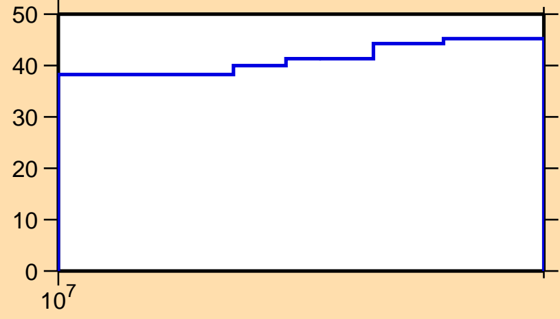
\Delta\sigma/\sigma vs. E for ^{49}\text{V}(n,2n)
