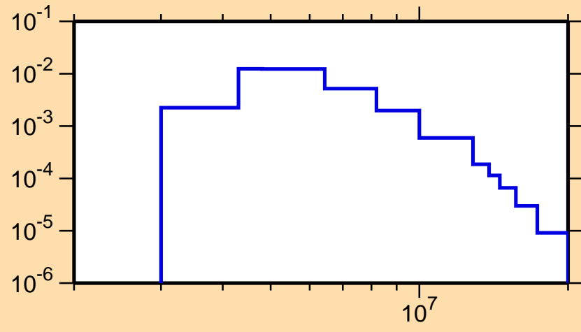
\sigma vs. E for ^{54}\text{Cr}(n,n_{14})
