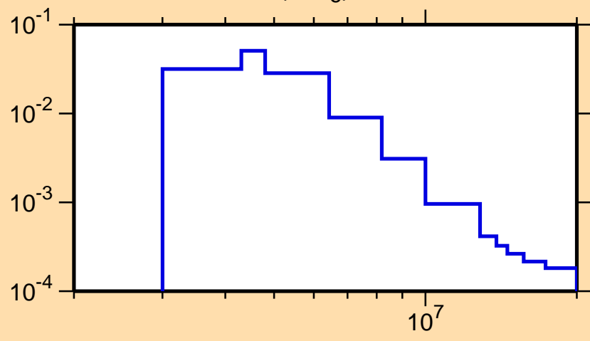
\sigma vs. E for ^{54}\text{Cr}(n,n_6)
