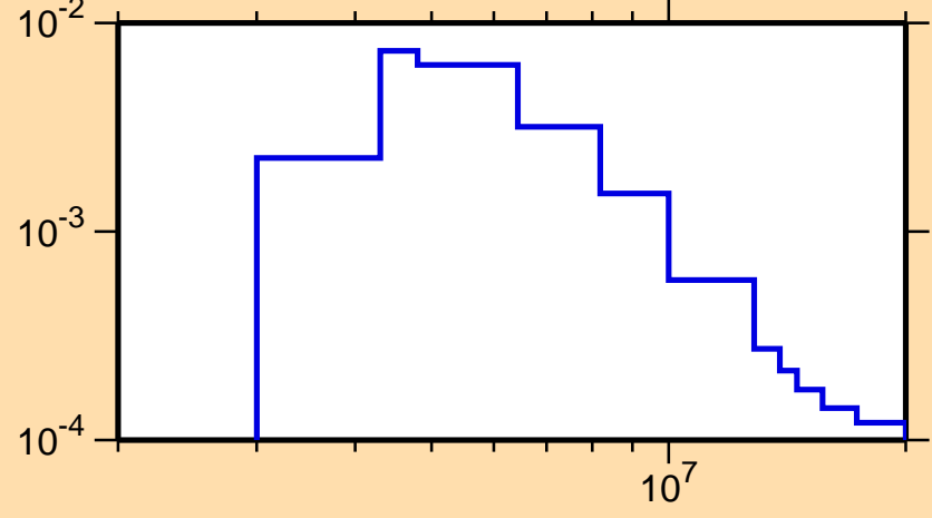
\sigma vs. E for ^{54}\text{Cr}(n,n_7)
