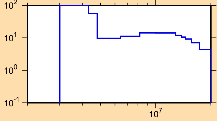
\Delta\sigma/\sigma vs. E for ^{54}\text{Cr}(\text{mt } 5)
