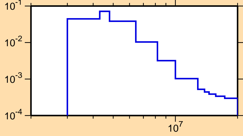
\sigma vs. E for ^{54}\text{Cr}(n,n_9)
