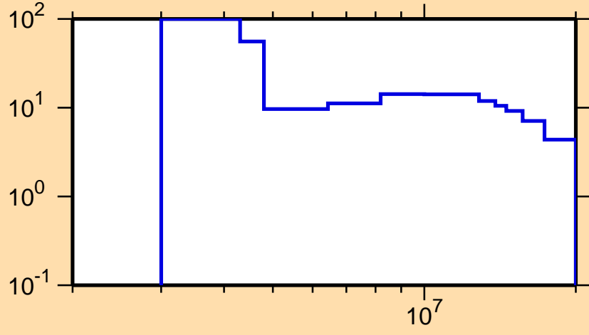
\Delta\sigma/\sigma vs. E for ^{54}\text{Cr}(\text{mt } 5)
