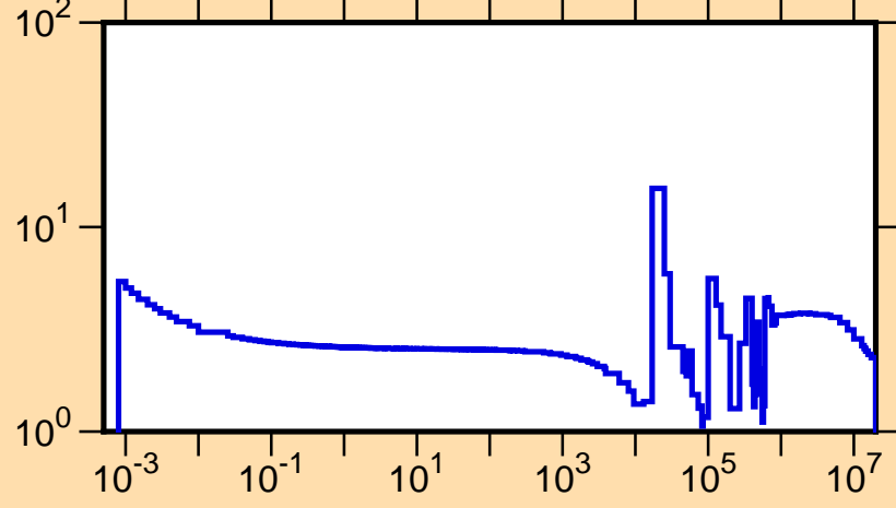
\sigma vs. E for ^{54}\text{Cr}(n,\text{tot.})
