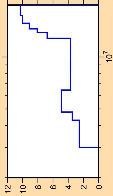
\Delta\sigma/\sigma vs. E for ^{54}\text{Cr}(n,n_6)
