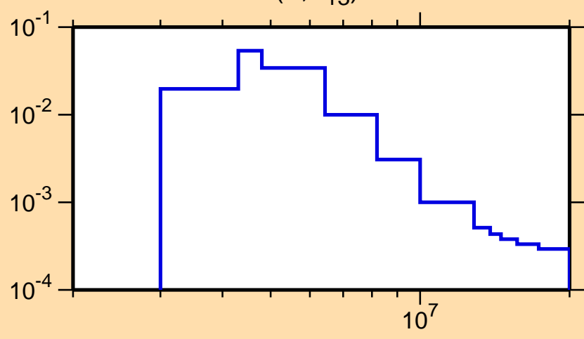
\sigma vs. E for ^{54}\text{Cr}(n,n_{13})
