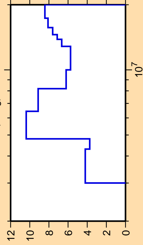
\Delta\sigma/\sigma vs. E for ^{54}\text{Cr}(n,n_5)
