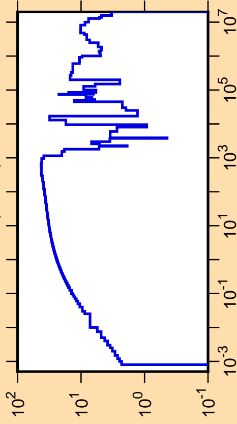
\Delta\sigma/\sigma vs. E for ^{49}\text{Ti}(n,\text{tot.})
