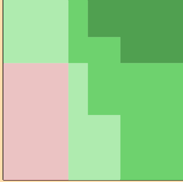
\Delta\sigma/\sigma vs. E for ^{51}\text{V}(n,2n)
