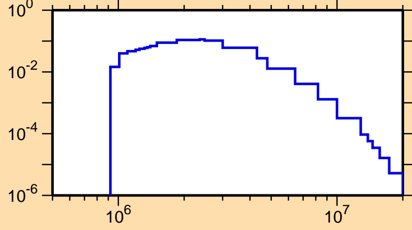
\sigma vs. E for ^{51}\text{V}(n,n_3)
