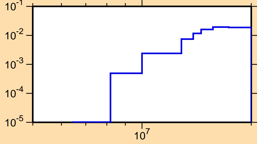
\sigma vs. E for ^{50}\text{Ti}(n,p)
