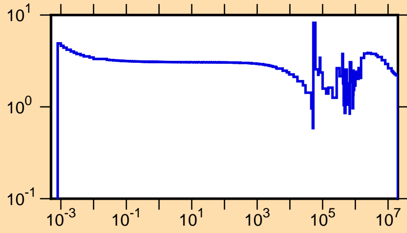
\sigma vs. E for ^{50}\text{Ti}(n,\text{tot.})
