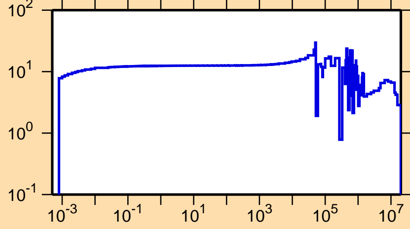
\Delta\sigma/\sigma vs. E for ^{50}\text{Ti}(n,\text{tot.})
