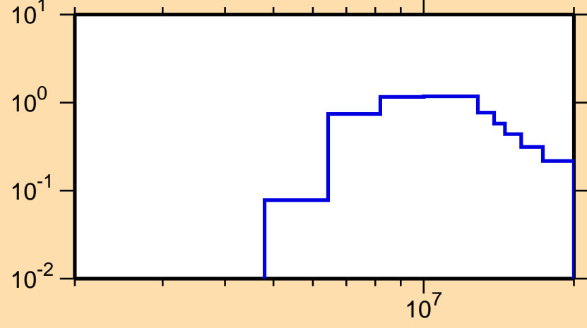
\sigma vs. E for ^{50}\text{Ti}(n,n\text{cont.})
