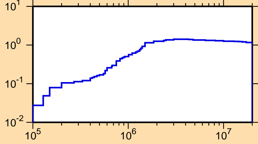
\sigma vs. E for ^{45}\text{Sc}(n,\text{nonel.})
