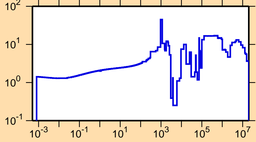
\Delta\sigma/\sigma vs. E for ^{45}\text{Sc}(n,\text{tot.})
