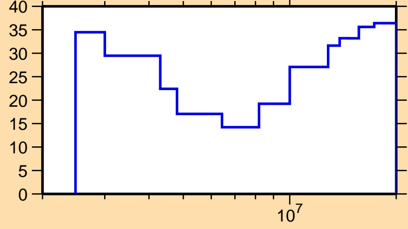
\Delta\sigma/\sigma vs. E for ^{48}\text{Sc}(n,ncont.)
