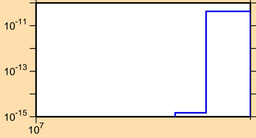
\sigma vs. E for ^{48}\text{Sc}(n,p\alpha)
