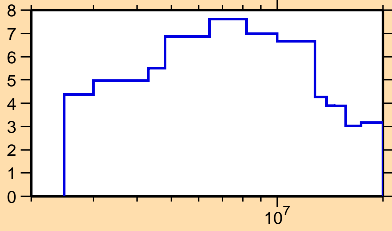
\Delta\sigma/\sigma vs. E for ^{48}\text{Sc}(n,tot.)
