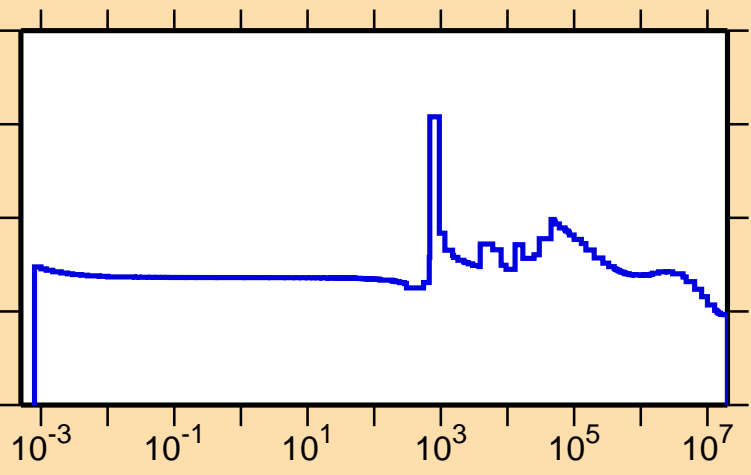
\sigma vs. E for ^{48}\text{Sc}(n,\text{el.})
