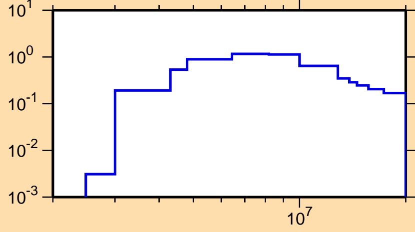
\sigma vs. E for ^{48}\text{Sc}(n,n\text{cont.})
