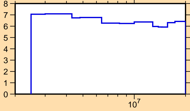
\Delta\sigma/\sigma vs. E for ^{48}\text{Sc}(n,\text{nonel.})
