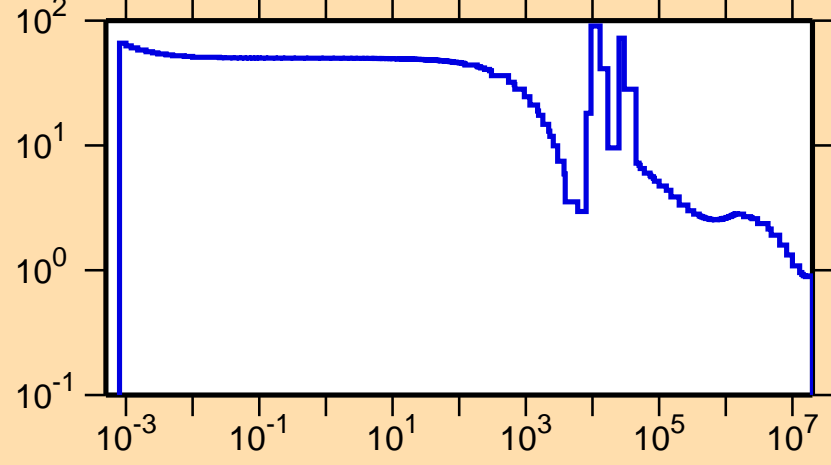
\sigma vs. E for ^{45}\text{Ca}(n,\text{el.})
