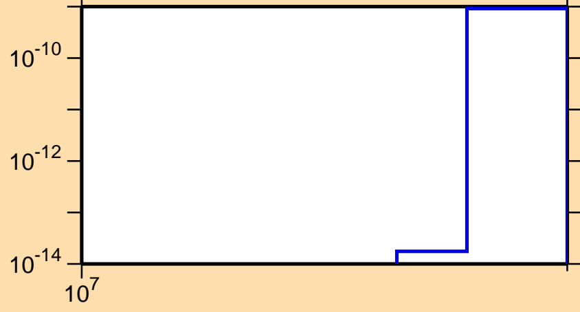
\sigma vs. E for ^{45}\text{Ca}(n,\text{He}3)
