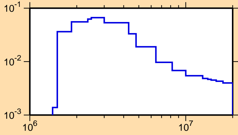
\sigma vs. E for ^{45}\text{Ca}(n,n_2)
