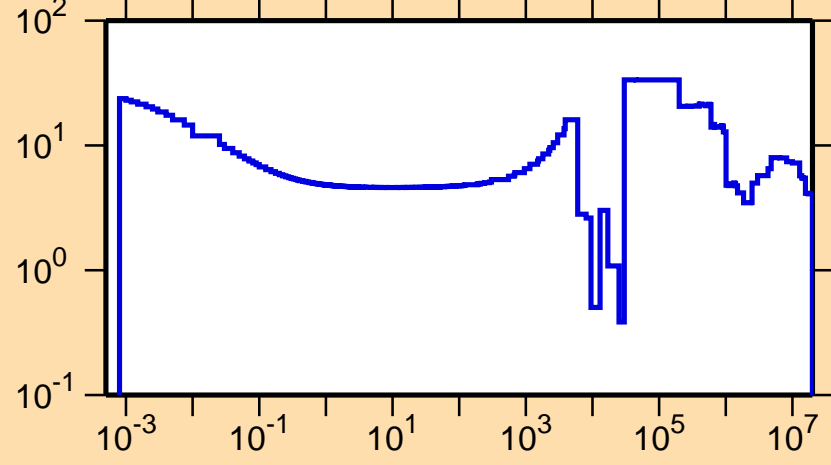
\Delta\sigma/\sigma vs. E for ^{45}\text{Ca}(n,\text{tot.})
