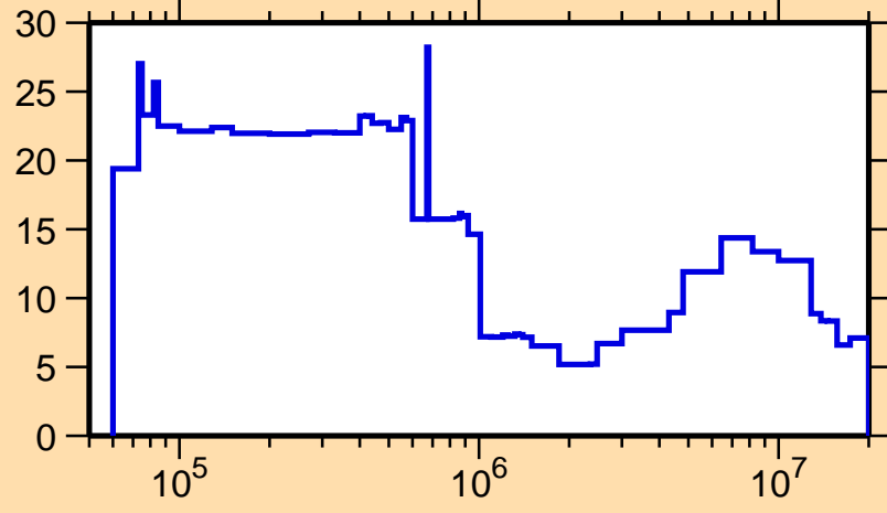
\Delta\sigma/\sigma vs. E for ^{41}\text{Ca}(n,el.)
