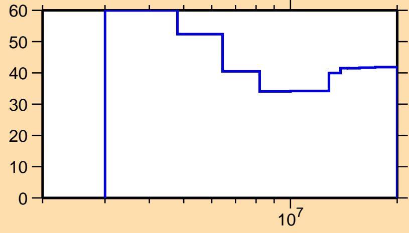
\Delta\sigma/\sigma vs. E for ^{41}\text{Ca}(n,n\text{cont.})
