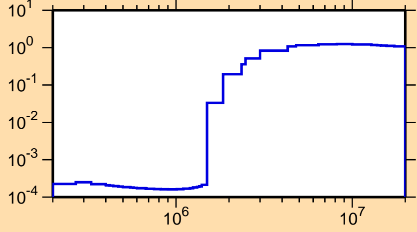
\sigma vs. E for ^{35}\text{S}(n,\text{nonel.})
