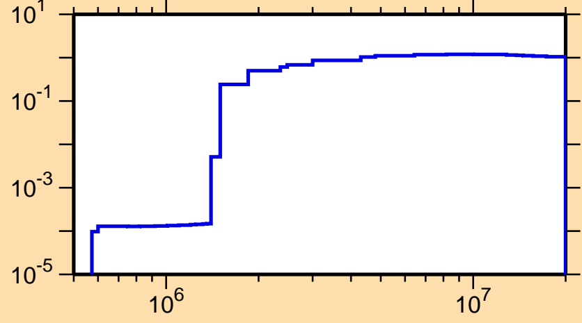
\sigma vs. E for ^{33}\text{P}(n,\text{nonel.})
