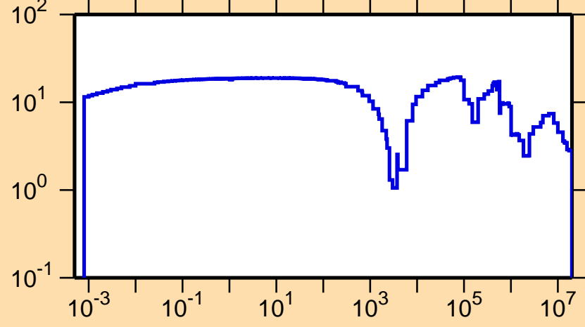
\Delta\sigma/\sigma vs. E for ^{33}\text{P}(n,\text{tot.})
