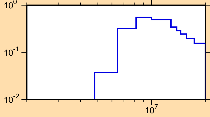
\sigma vs. E for ^{33}\text{S}(n,n\text{cont.})
