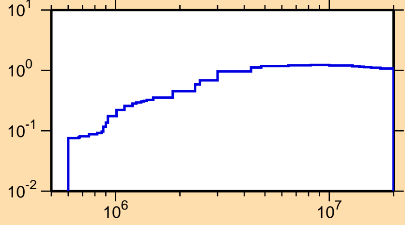
\sigma vs. E for ^{33}\text{S}(n,\text{nonel.})
