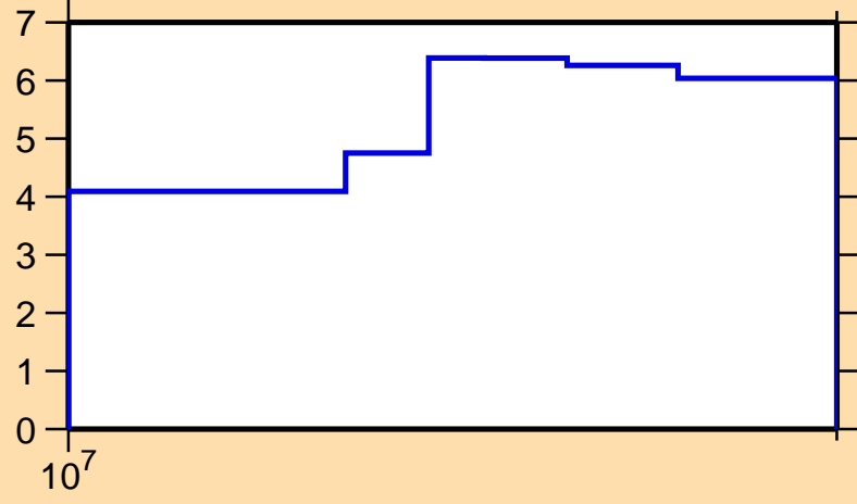
\Delta\sigma/\sigma vs. E for ^{32}\text{Si}(n,el.)
