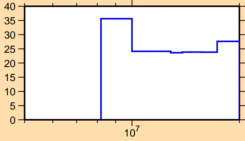
\Delta\sigma/\sigma vs. E for ^{32}\text{Si}(n,n\text{cont.})
