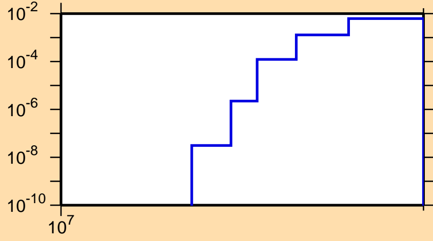
\sigma vs. E for ^{32}\text{Si}(n,n\alpha)
