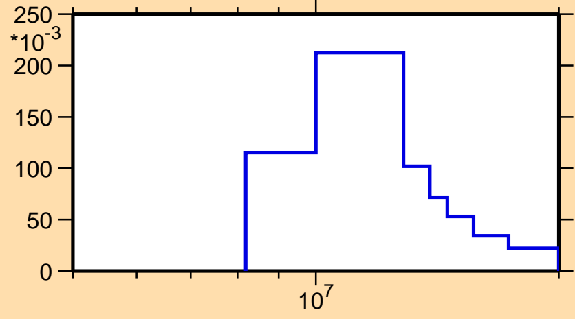
\sigma vs. E for ^{32}\text{Si}(n,n\text{cont.})
