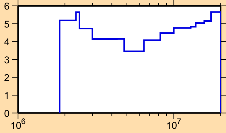
\Delta\sigma/\sigma vs. E for ^{32}\text{Si}(n,\text{nonel.})
