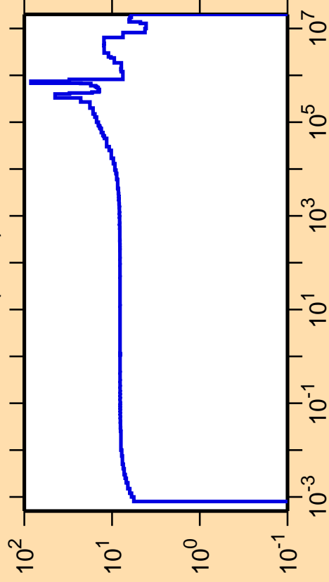
\Delta\sigma/\sigma vs. E for ^{32}\text{Si}(n,\text{el.})
