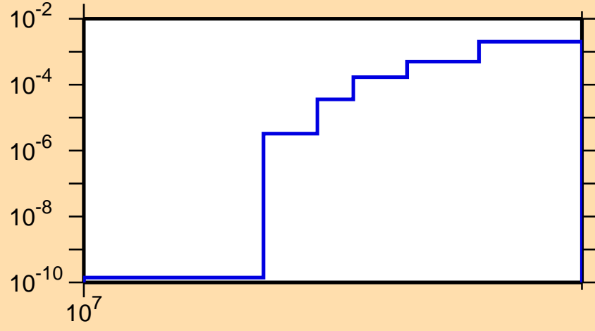
\sigma vs. E for ^{32}\text{Si}(n,p)
