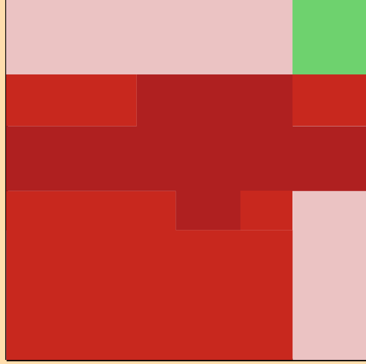
\Delta\sigma/\sigma vs. E for ^{32}\text{Si}(n,\gamma)
