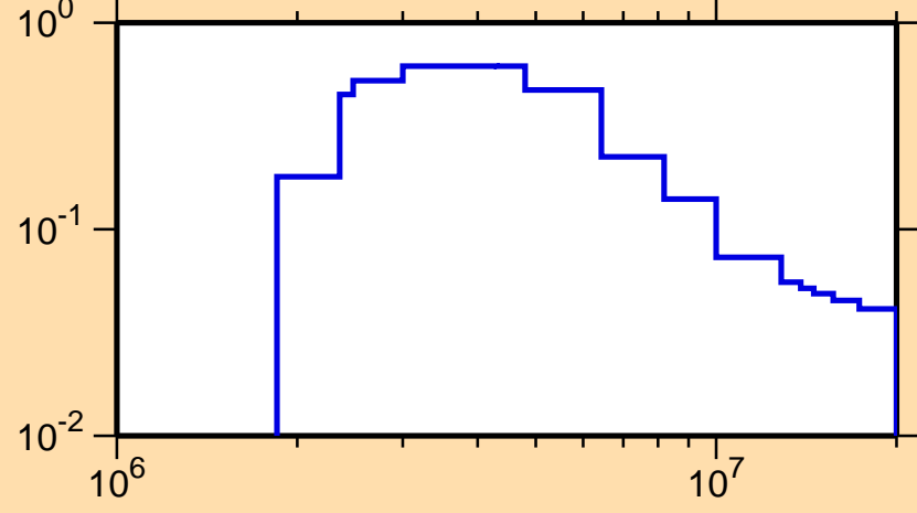
\sigma vs. E for ^{32}\text{Si}(n,n_1)
