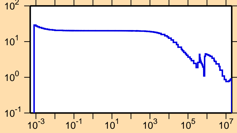
\sigma vs. E for ^{32}\text{Si}(n,\text{el.})
