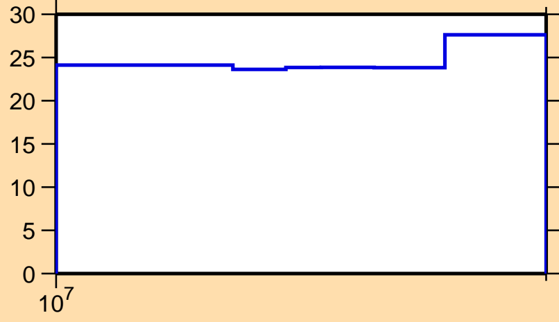
\Delta\sigma/\sigma vs. E for ^{32}\text{Si}(n,ncont.)
