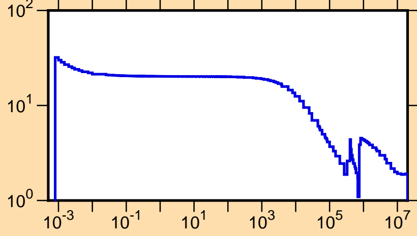
\sigma vs. E for ^{32}\text{Si}(n,\text{tot.})
