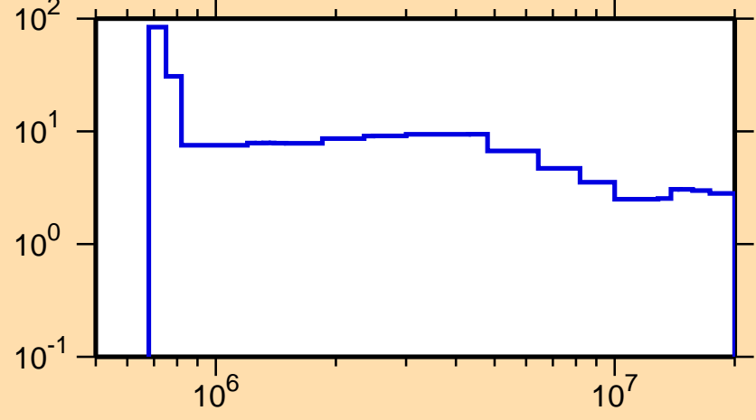
\Delta\sigma/\sigma vs. E for ^{32}\text{Si}(n,\text{tot.})
