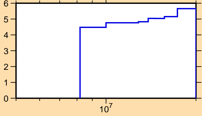
\Delta\sigma/\sigma vs. E for ^{32}\text{Si}(n,n\text{nonel.})
