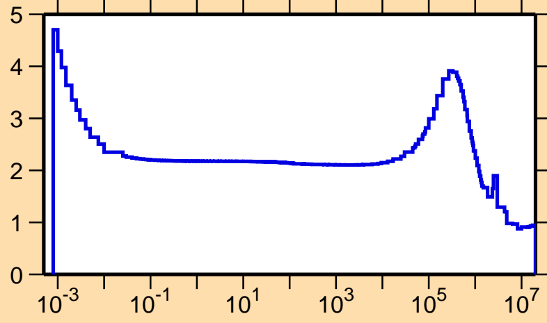
\sigma vs. E for ^{10}\text{B}(n,\text{el.})
