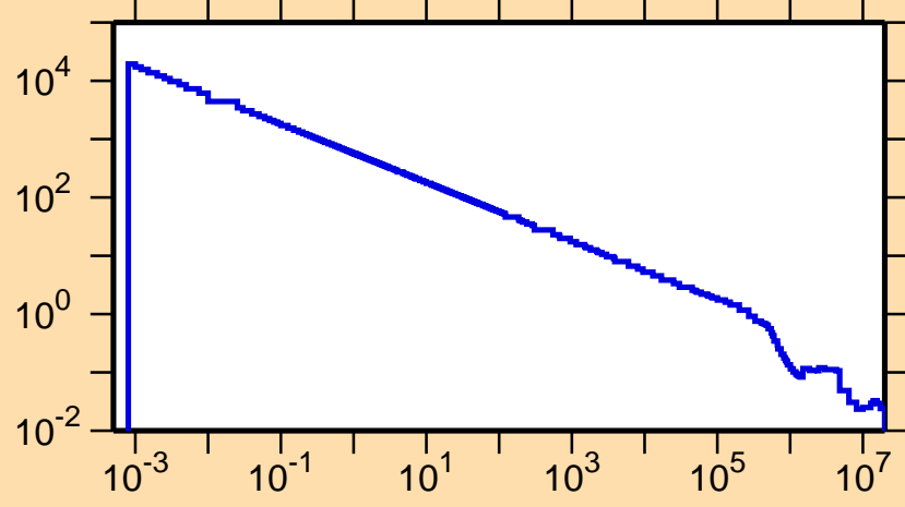
\sigma vs. E for ^{10}\text{B}(n,a_1)
