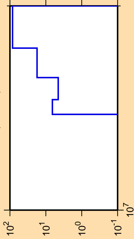
\Delta\sigma/\sigma vs. E for {}^7\text{Li}(\text{mt858})
