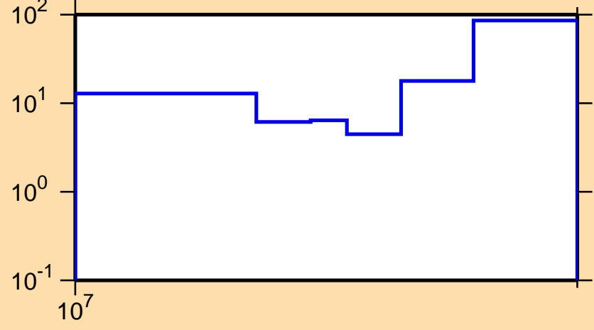
\Delta\sigma/\sigma vs. E for {}^7\text{Li}(\text{mt855})
