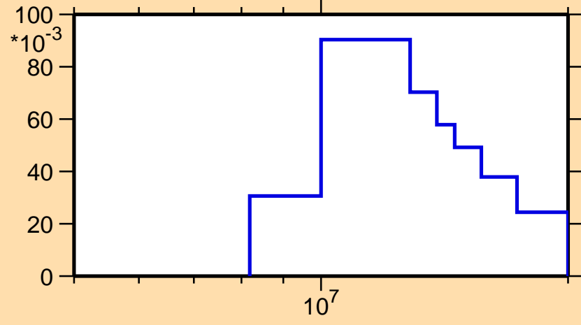
\sigma vs. E for {}^7\text{Li}(\text{mt856})
