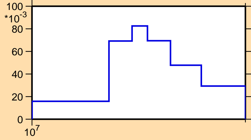
\sigma vs. E for {}^7\text{Li}(\text{mt857})
