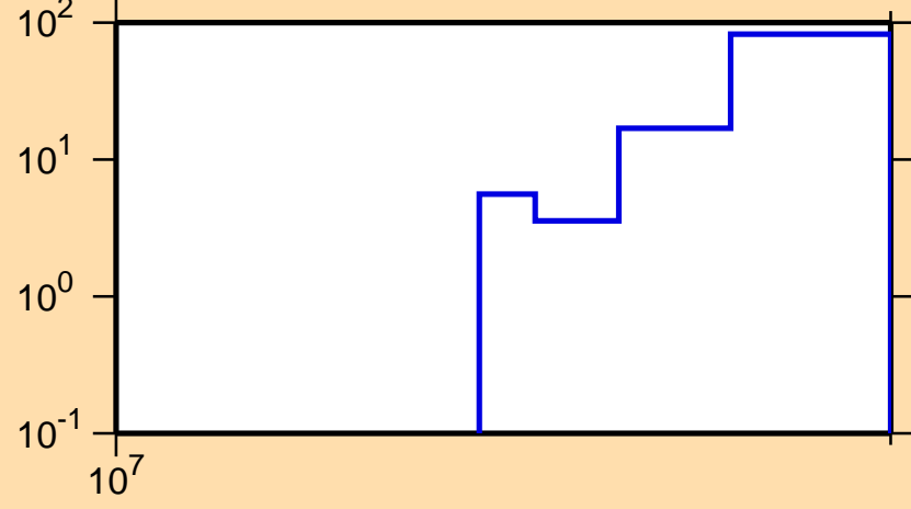
\Delta\sigma/\sigma vs. E for {}^7\text{Li}(\text{mt854})
