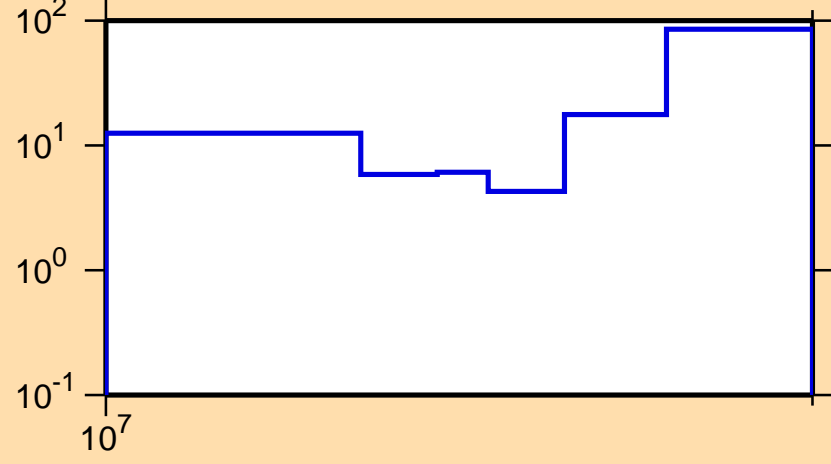
\Delta\sigma/\sigma vs. E for {}^7\text{Li}(\text{mt856})
