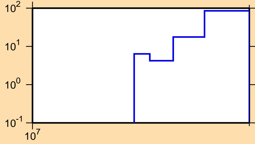
\Delta\sigma/\sigma vs. E for {}^7\text{Li}(\text{mt857})
