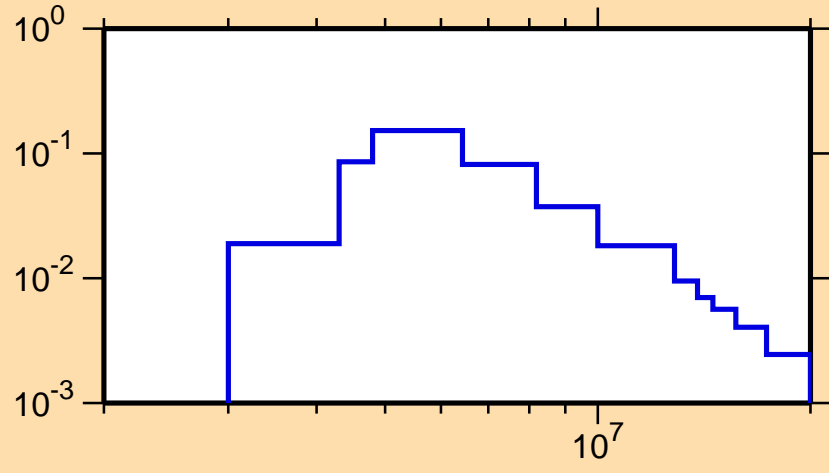
\sigma vs. E for {}^7\text{Li}(\text{mt853})
