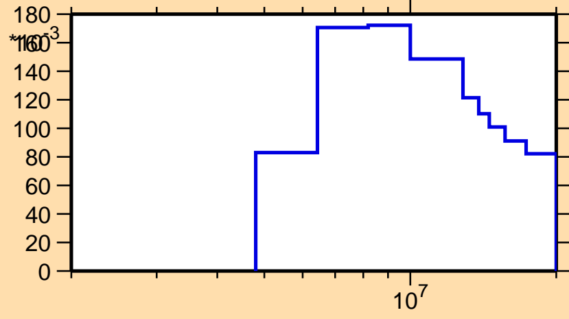
\sigma vs. E for {}^7\text{Li}(\text{mt854})
