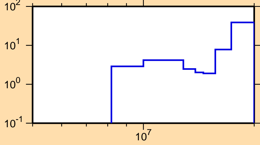
\Delta\sigma/\sigma vs. E for {}^7\text{Li}(\text{n,inel.})
