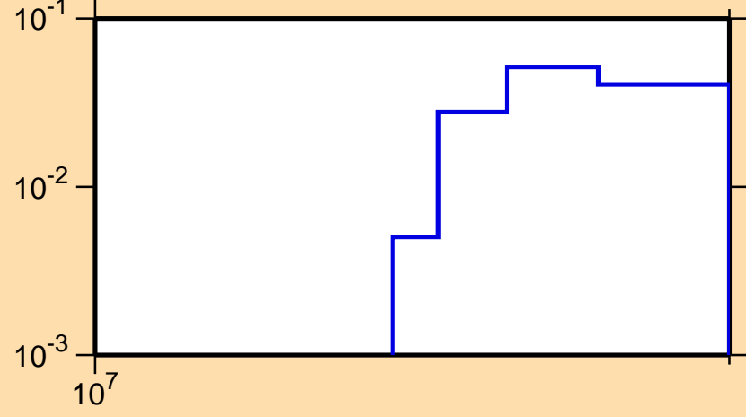
\sigma vs. E for {}^7\text{Li}(\text{mt858})
