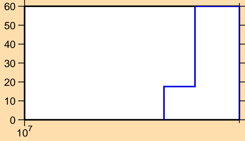
\Delta\sigma/\sigma vs. E for {}^7\text{Li}(\text{mt858})
