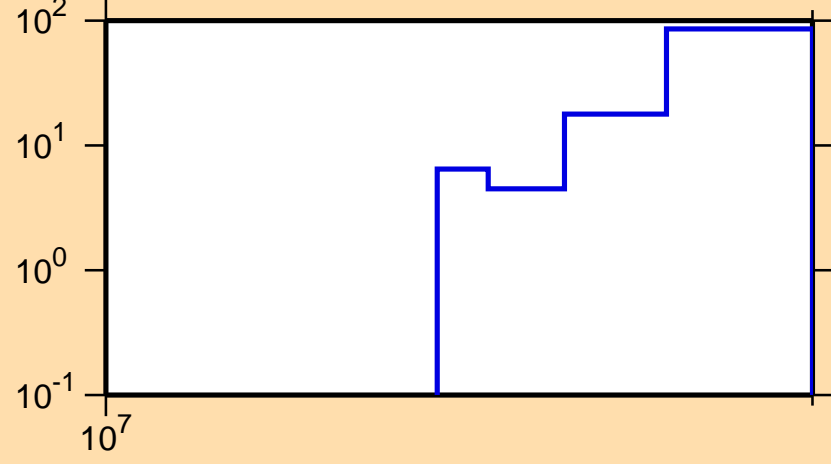
\Delta\sigma/\sigma vs. E for {}^7\text{Li}(\text{mt853})
