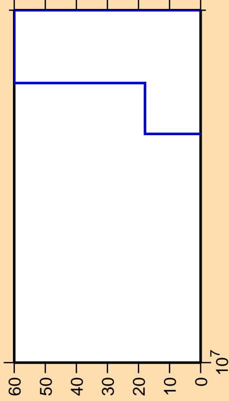
\Delta\sigma/\sigma vs. E for {}^7\text{Li}(\text{mt859})
