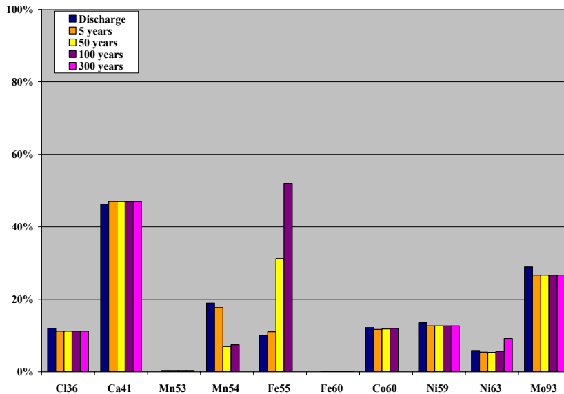
Figure 5: RSD results for Activation Products in cell calculations
