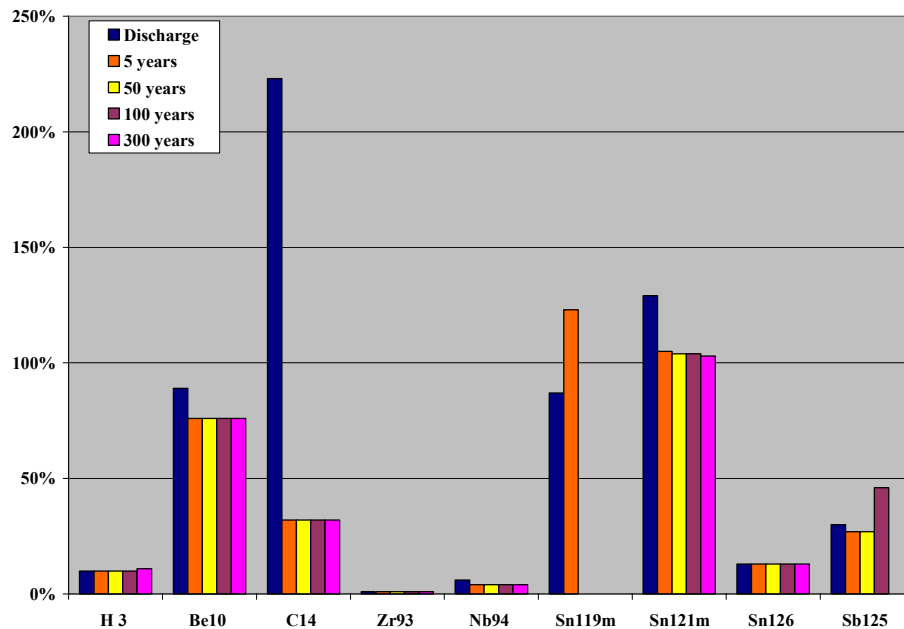
Figure 6: RSD results for Activation-Fission Products in assembly calculations
