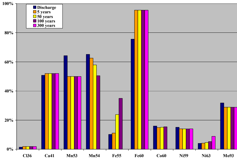
Figure 5: RSD results for Activation Products in cell calculations
