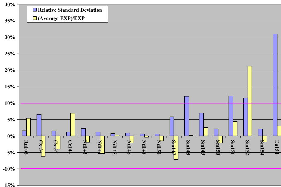
Figure 2: Results for fission products; comparison of calculated average values to measured values
