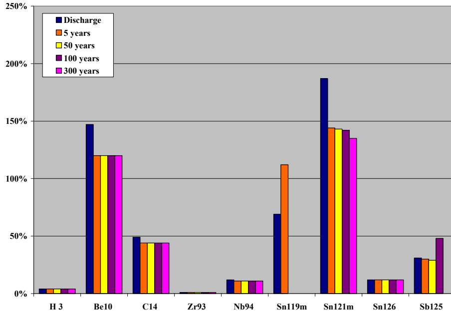
Figure 7: RSD results for Activation-Fission Products in cell calculations
