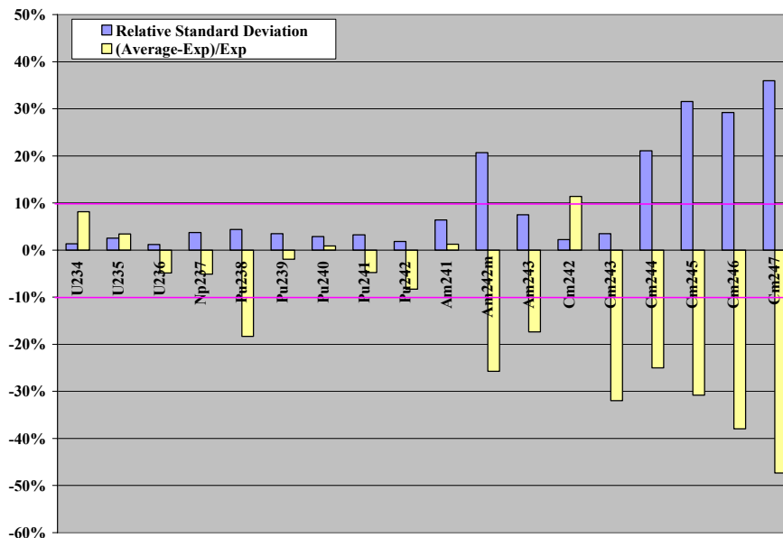
Figure 1: Results for actinides; comparison of calculated average values to measured values
