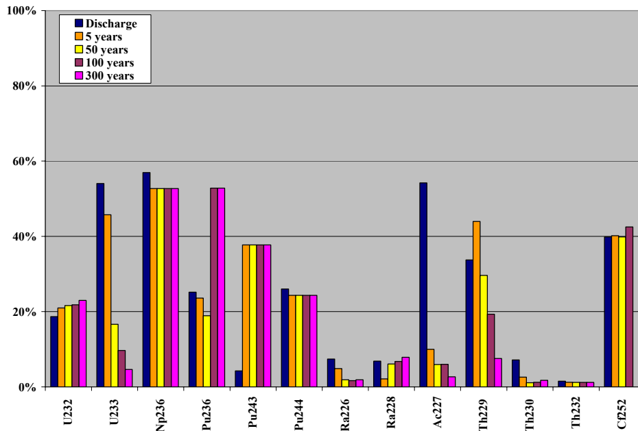
Figure 3: Results of Relative Standard Deviation versus cooling time for actinides
