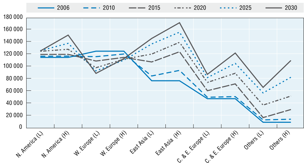
Figure 3. PROJECTED INSTALLED NUCLEAR CAPACITY TO 2030 Low and high projections
