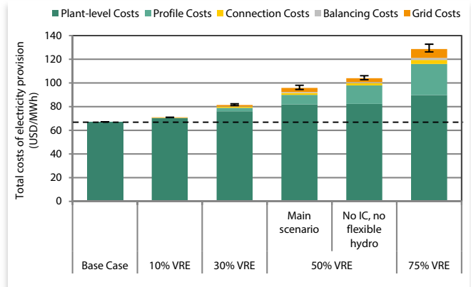
Figure 1: Total cost of electricity at different shares of VREs
