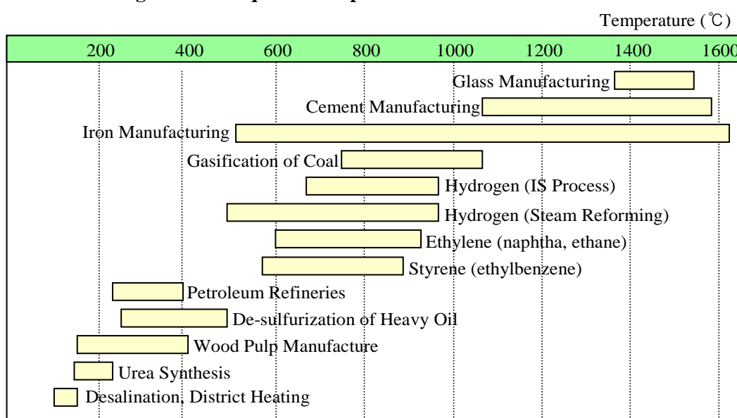
Figure 1. Required Temperature for Industrial Processes
