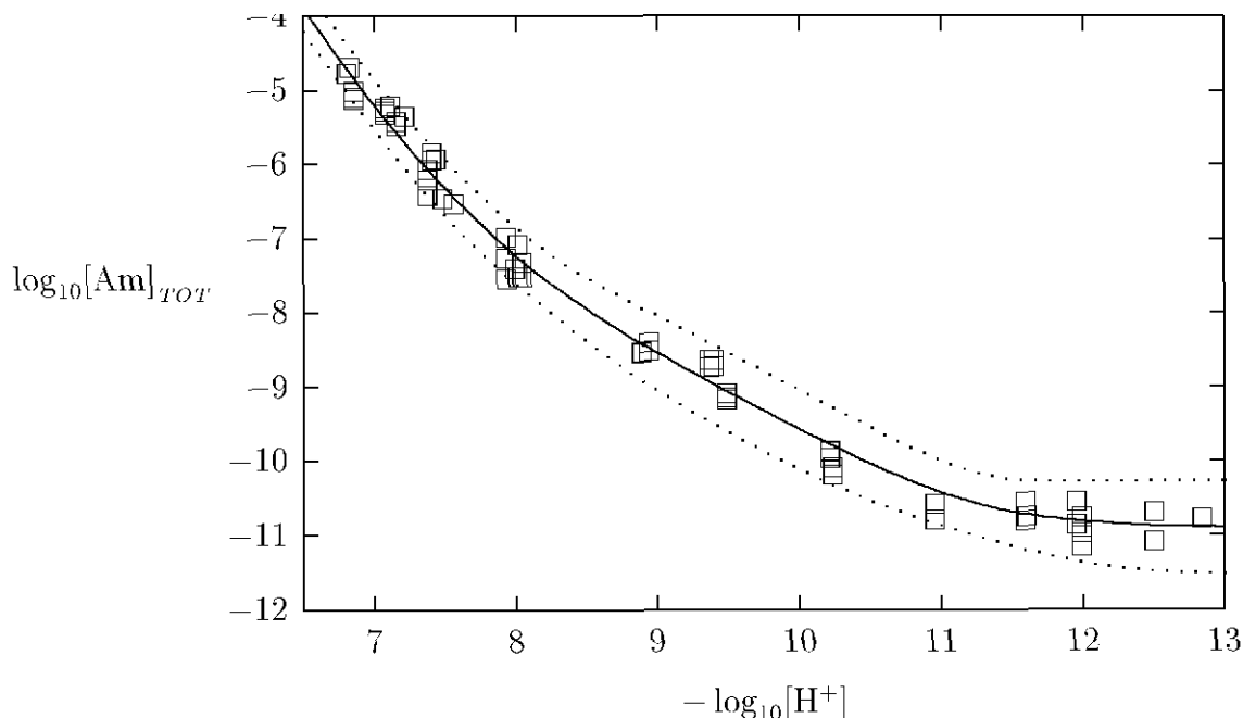
Figure A.9: Solubility measurements of Am(III) hydroxide in 0.1 M NaClO 4 and 25°C from Stadler and Kim [88STA/KIM]. Tllc continuous curve represents the solubility values calculated with the set of equilibrium constants re-estimated by this review from experimental data in Ref. [88STA/KIM] and the dotted curves show the associated uncertainties.
