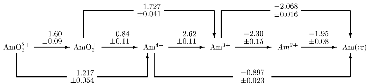
Figure 1 : Electrode potentials (in units of V) for some americium redox couples. The species \text{Am}^{2+} is italicized to stress the fact that it is only a transient species, cf. Section V.2.1.
