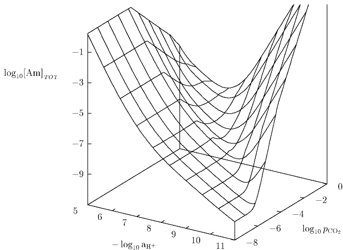
Figure V.13: Calculated solubility diagram for the americium(III) hydroxide-carbonate system in the range 5 \leq \text{pH} \leq 11 and -8 \leq \log_{10} p_{\text{CO}_2} \leq 0 , at 25°C and standard conditions ( \mathbf{I} = 0 ).
