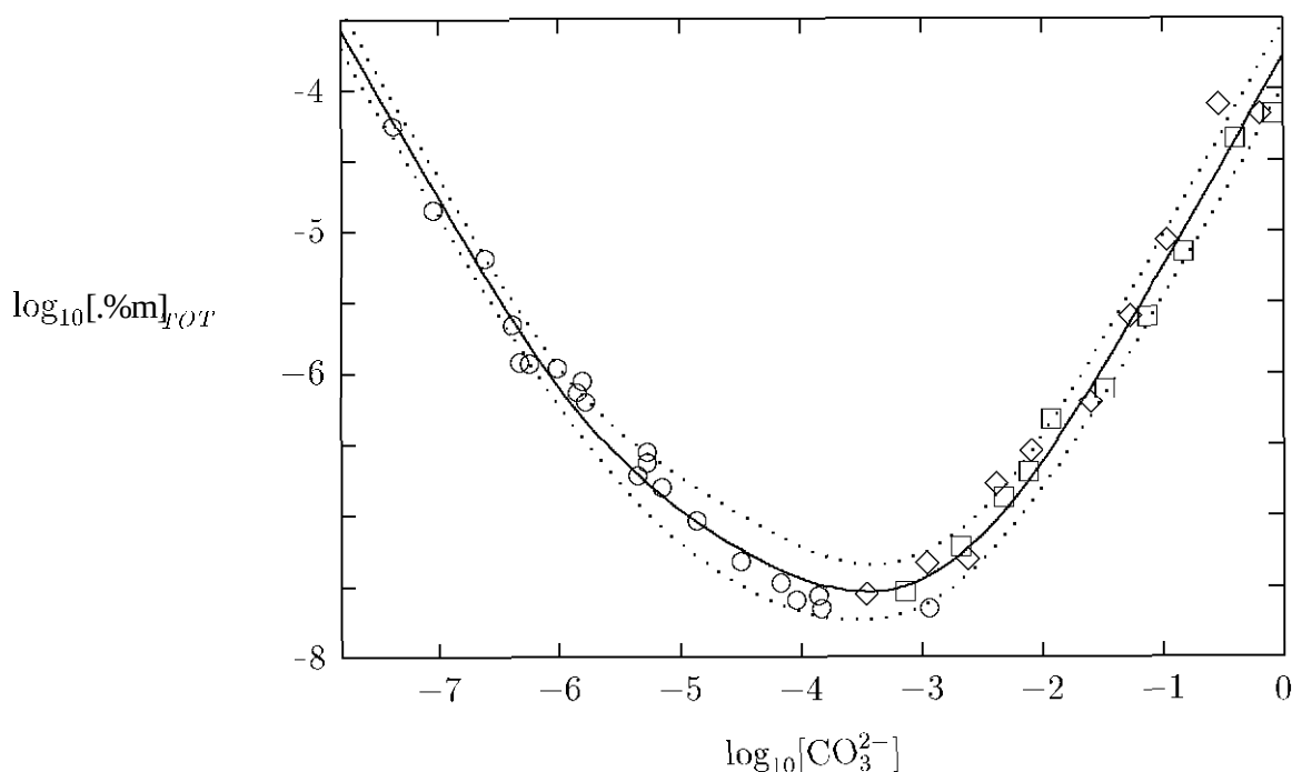
Figure A.10: Solubility measurements of Am(III) at 3 M NaClO 4 and 20°C from Robouch [89ROB]. The diagram shows experimental points (○) obtained under controlled CO 2 (g) partial pressure (0.1, 0.3 and 1.0 atm) and data from batch experiments sampled after 10 and 20 weeks of equilibration time (◇ and □ respectively). The continuous curve represents the solubility of Am 2 (CO 3 ) 3 (cr) calculated with the set of equilibrium constants re-estimated by this review from data in Ref. [89ROB], and the dotted curves show the associated uncertainty.
