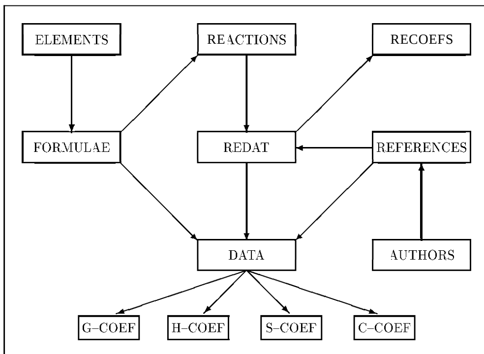
Figure 11.2: Principal schema of the NEA Thermochemical Data Base.
