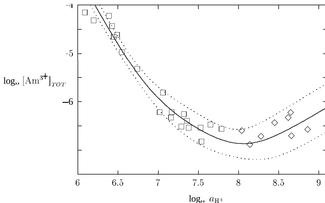
Figure -4.13: Solubility measurements of \text{Am}_2(\text{CO}_3)_3(\text{cr}) from Meinrath and Kim [91MEI/KIM] at 0.1 M \text{NaClO}_4 and \text{pH} < 8 ( \square ) and 0.3 M \text{NaClO}_4 and \text{pH} \geq 8 ( \circ ) and at p_{\text{CO}_2} = 0.01 atm and 25^\circ\text{C} . The continuous curve represents the values calculated with the set of equilibrium constants determined by Meinrath and Kim [91MEI/KIM], and the dotted curves show the associated uncertainty.
