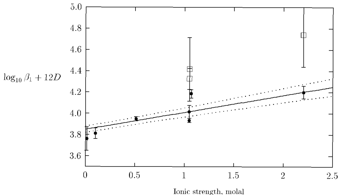
Figure V.9: Extrapolation to I = 0 of experimental data for the equilibrium constants of formation of \text{AmSO}_4^+ , according to reaction (V.23), using the specific ion interaction equations ( cf. Appendix B). Both experiments with [\text{H}^+] \geq 1 \text{ M} ( \square ) and [\text{H}^+] \leq 1 \text{ mM} ( \bullet ) are plotted. The result of the weighted linear regression for the experiments with [\text{H}^+] \leq 1 \text{ mM} is shown as a straight line, and the dotted lines represent the uncertainty range.
