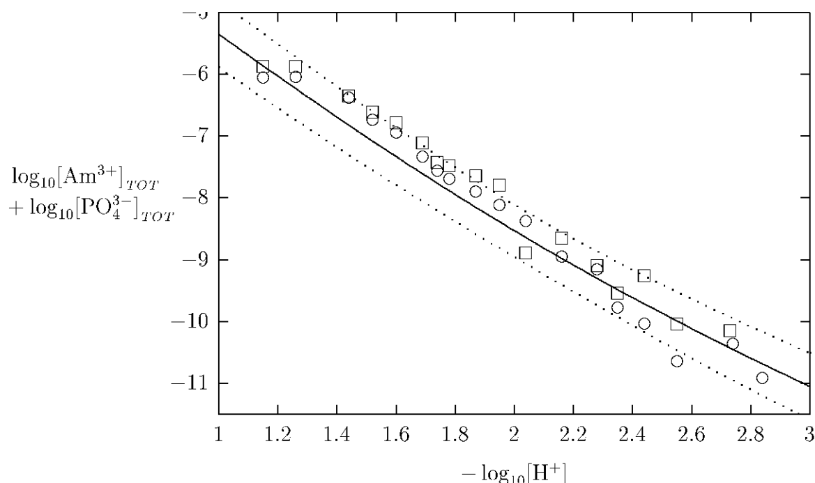
Figure A.14: Solubility measurements of \text{AmPO}_4 \cdot x\text{H}_2\text{O}(\text{am}) from Rni. Fclmy and Fulton [92RAI/FEL] (at 21 days, \square , and 86 days, \circ , equilibration time). The continuous curve represents the values calculated with the solubility product reported in [92RAI/FEL] ( i.e. \log_{10} K_{s,0}^\circ = -24.79 ) in combination with the selected acidity constants for phosphoric acid given in Table IV.2 and the specific ion interaction equations in Appendix B. The dotted curves show the calculated uncertainty on the solubility when the uncertainty in the value of \log_{10} K_{s,0}^\circ is set to \pm 0.6 .
