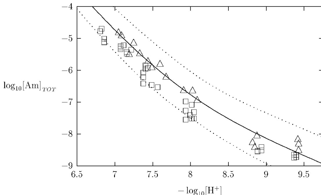
Figure A.3: Solubility measurements of Am(III) hydroxide in 0.1 M NaClO 4 from Silva [82SIL] (A) and from Ref. [88STA/KIM] (U). The continuous curve represents the values calculated with the set of equilibrium constants re-estimated by this review from experimental data in Ref. [82SIL], and the dotted curves show the associated uncertainties.
