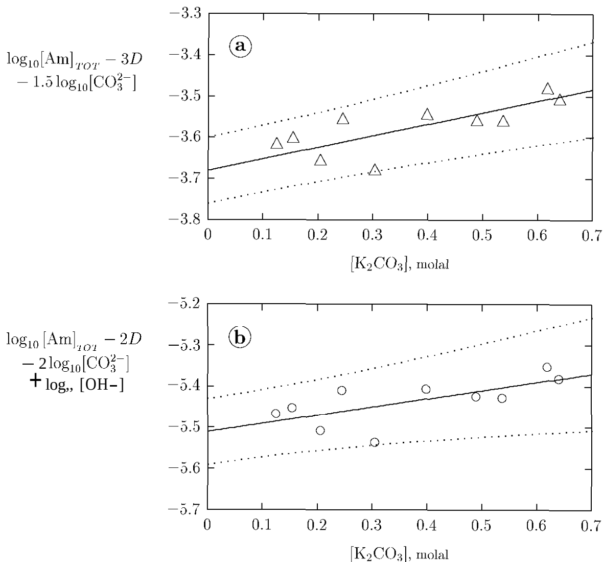
Figure 1 : Experimental solubility data from [69SHI/GIV] extrapolated to I = 0 using the specific ion interaction equations (cf. Appendix B). Upper diagram (a) assuming reaction: 0.5\text{Am}_2(\text{CO}_3)_3(\text{s}) + 1.5\text{CO}_3^{2-} \rightleftharpoons \text{Am}(\text{CO}_3)_3^{3-} . Lower diagram (b) assuming reaction: \text{AmCO}_3\text{OH}(\text{s}) + 2\text{CO}_3^{2-} \rightleftharpoons \text{Am}(\text{CO}_3)_3^{3-} + \text{OH}^- . The lines correspond to Eqs. (A.1) and (A.2) respectively, and the dotted curves represent the 95% confidence intervals.
