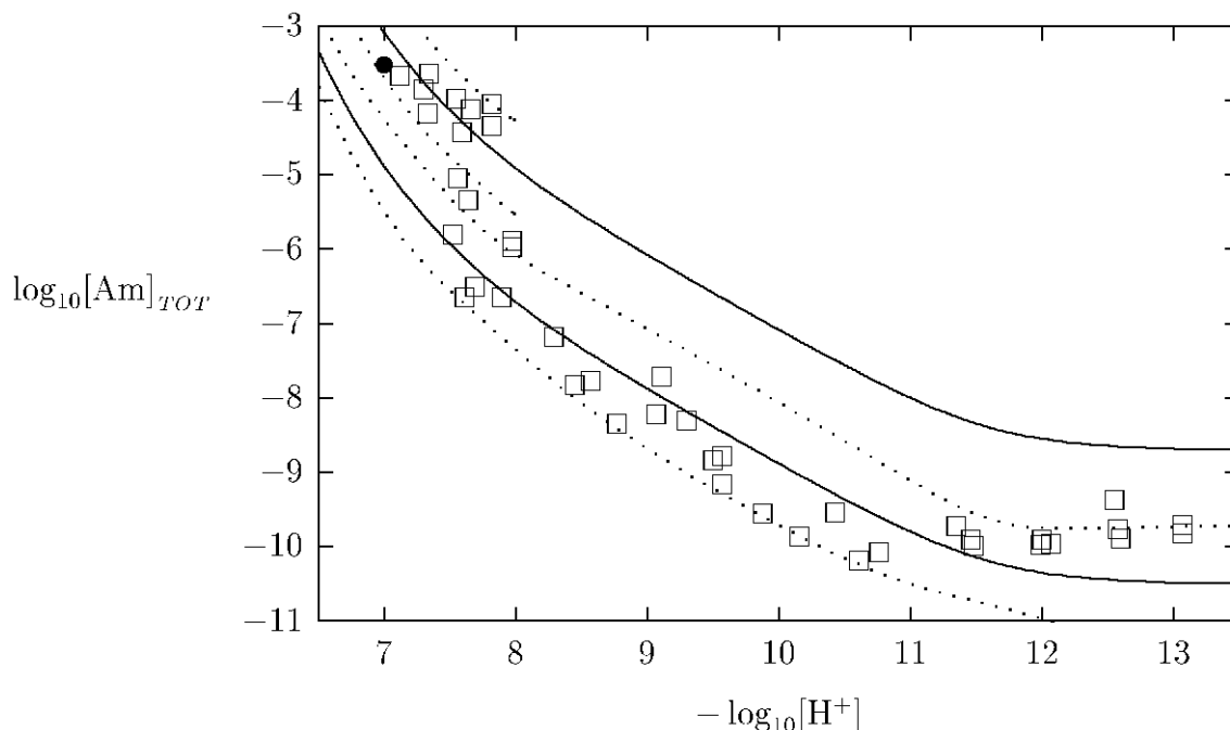
Figure A.4: Solubility measurements of amorphous Am(III) hydroxide from [83RAI/STR] in pH-adjusted deionized water ( \square ), and from [85NIT/EDE2] in 0.1 M NaClO 4 ( \bullet ). The continuous curves represents the values calculated with the selected set of hydrolysis constants (cf. Table 111.2) at low ionic strengths. The upper continuous curve corresponds to \log_{10}^* K_{s,0}^{\circ} = (17.0 \pm 0.6) ; and the lower one to \log_{10}^* K_{s,0}^{\circ} = (15.2 \pm 0.6) . The dotted curves show the associated uncertainties.
