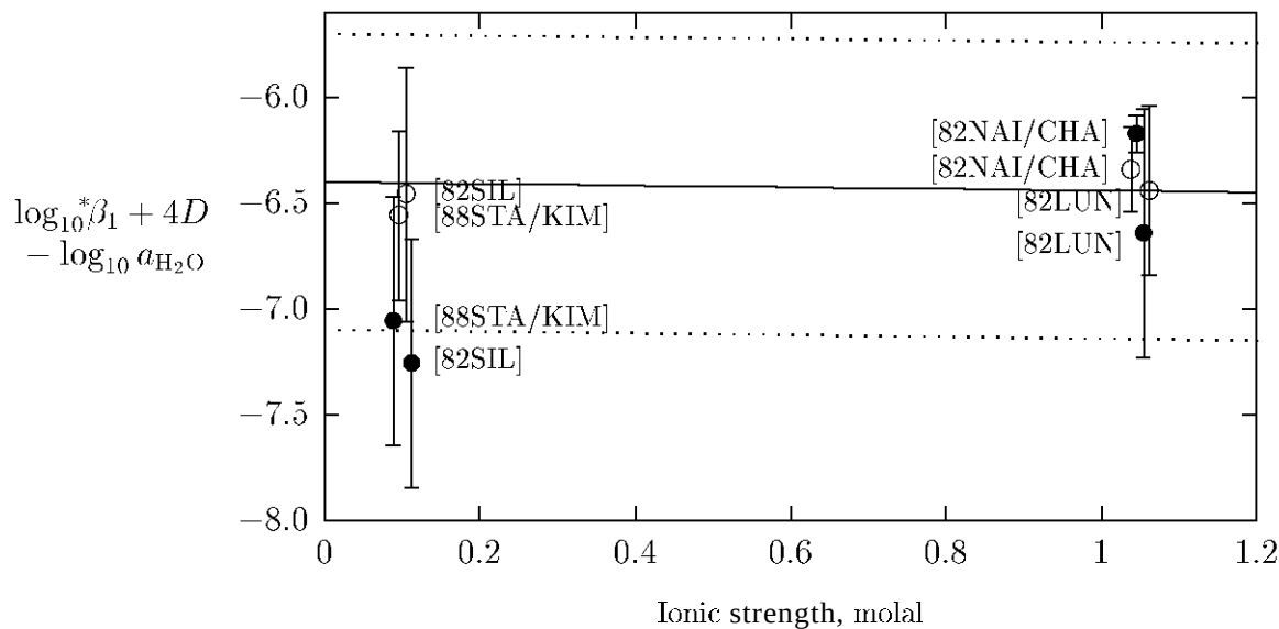
Figure V.4: Equilibrium constants for reaction: \text{Am}^{3+} + \text{H}_2\text{O}(\text{l}) \rightleftharpoons \text{AmOH}^{2+} + \text{H}^+ at 25°C in \text{NaClO}_4 solutions plotted according to Eq. (B.5). Open circles correspond to the values re-evaluated in this review and given in Table V.5, while filled circles correspond to the original values reported in the literature, cf. Table V.4 (with the uncertainties increased by a factor of 1.96 in order to approximate the 95% uncertainty level). For increased readability, the symbols are arbitrarily shifted ( \leq \pm 0.014 mol/kg) along the X-axis. The solid line represents Eq. (B.5) with \log_{10}^* \beta_1^\circ = -(6.4 \pm 0.2) and \Delta \varepsilon = (0.04 \pm 0.05) \text{ kg} \cdot \text{mol}^{-1} . The associated uncertainties are given by the dotted lines.
