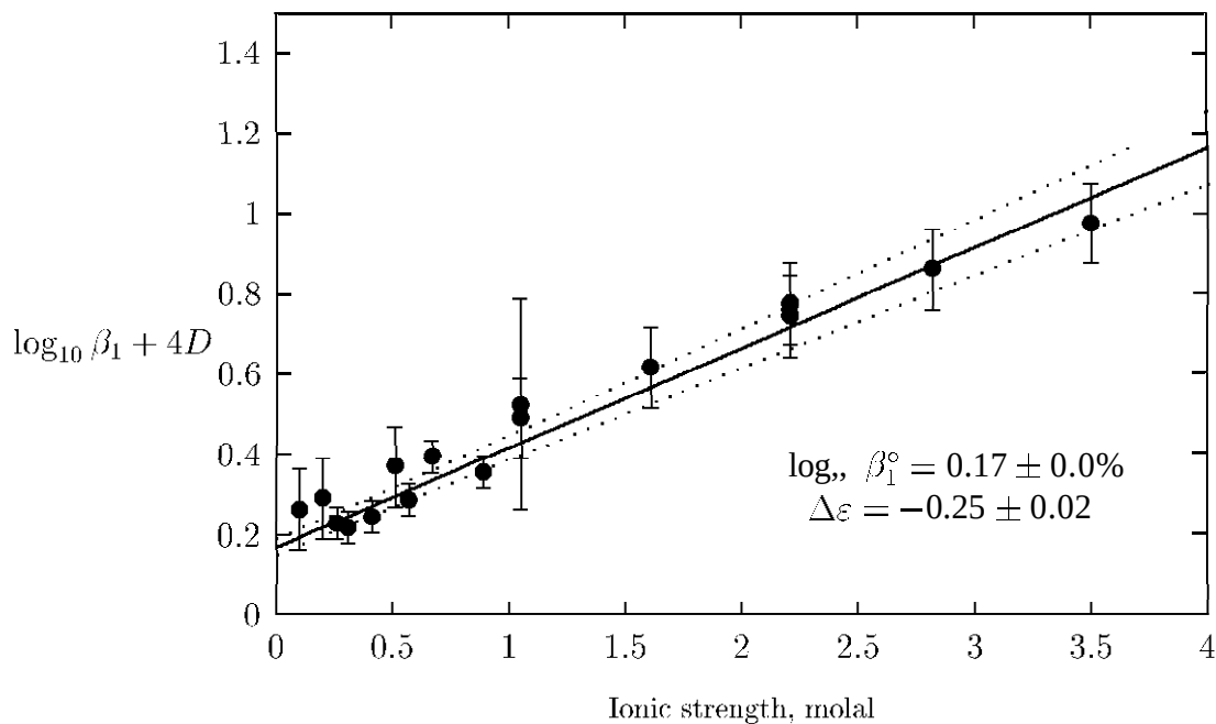
Figure B.1: Plot of \log_{10} \beta_1 + 4D vs. I , for Reaction (B.12), \text{UO}_2^{2+} + \text{Cl}^- \rightleftharpoons \text{UO}_2\text{Cl}^+ at, 25°C and 1 bar. The straight line shows the result of the weighted linear regression, and the dotted lines represent the uncertainty range obtained by propagating the resulting uncertainties at I = 0 back to I = 4 m.
