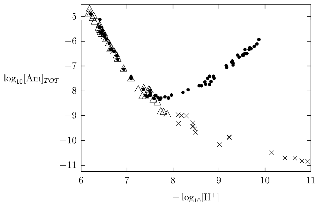
Figure A.6: Solubility data of americium(III) reported by Bernkopf and Kim [84BER/KIM] in the absence of \text{CO}_2(\text{g}) in 0.1 M \text{NaClO}_4 (A at \text{pH} < 8 . and \times at \text{pH} \geq 8 ) and at p_{\text{CO}_2} = 10^{-3.5} atm ( \bullet ) in 0.1 to 0.3 M \text{NaClO}_4 .
