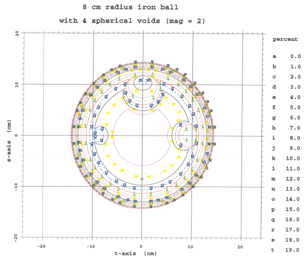
Figure 2. A million-pixel radiograph of an iron ball with four internal voids.
