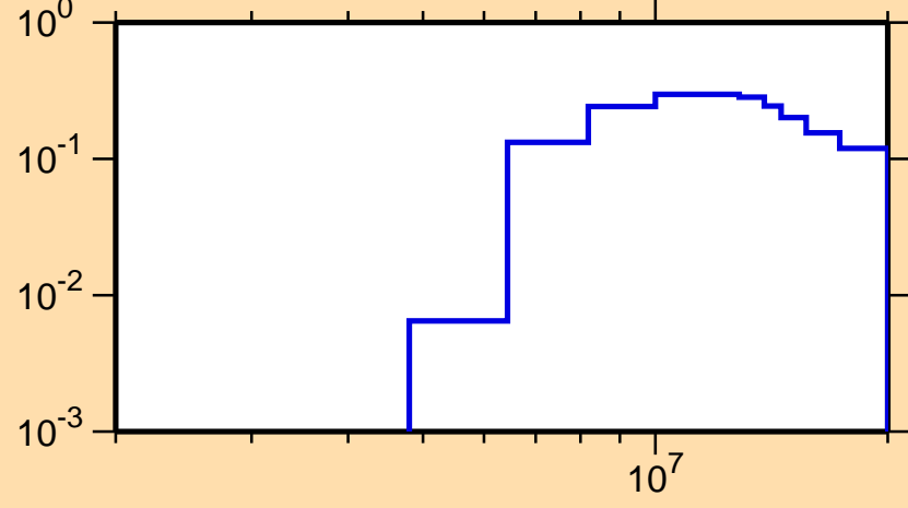
\sigma vs. E for ^{236}\text{Np}(n,2n)
