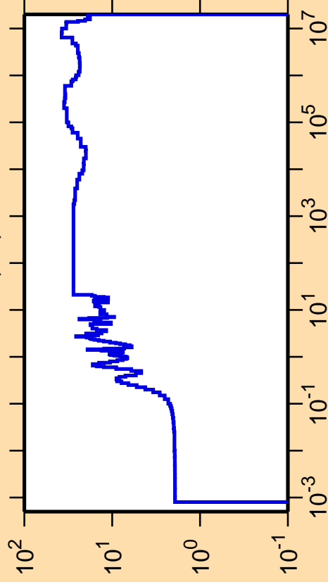
\Delta\sigma/\sigma vs. E for ^{232}\text{Pa}(n,f)
