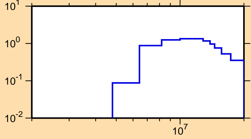
\sigma vs. E for ^{232}\text{Pa}(n,2n)
