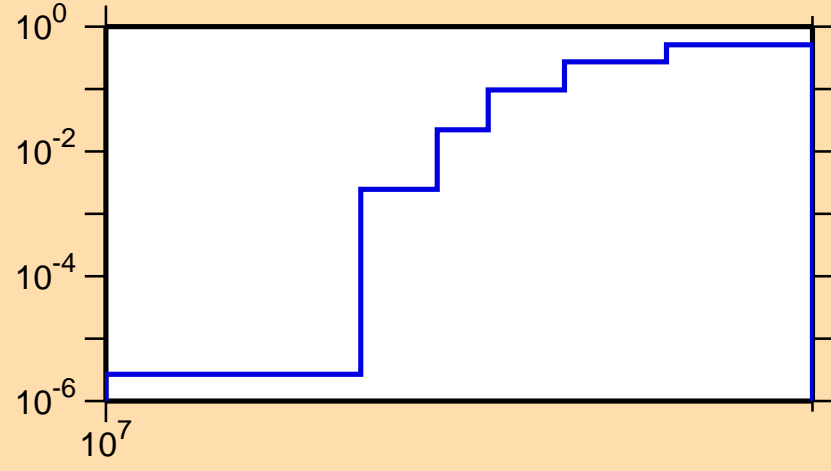
\sigma vs. E for ^{232}\text{Pa}(n,3n)
