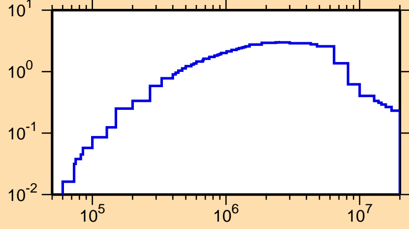
\sigma vs. E for ^{232}\text{Pa}(n,\text{inel.})
