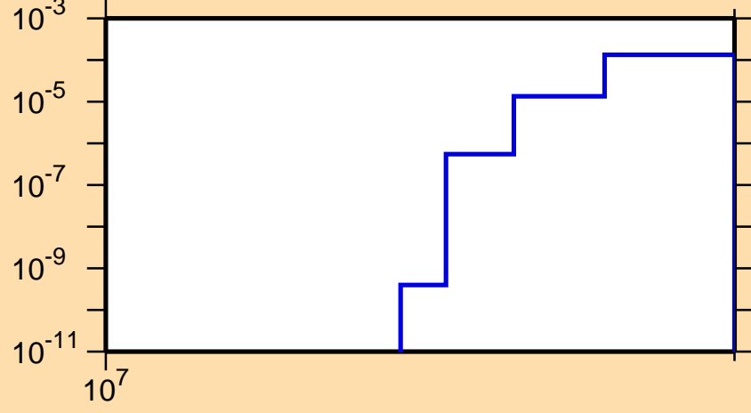
\sigma vs. E for ^{209}\text{Po}(n,2np)
