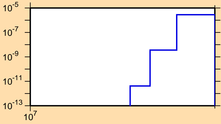
\sigma vs. E for ^{209}\text{Po}(n,nt)
