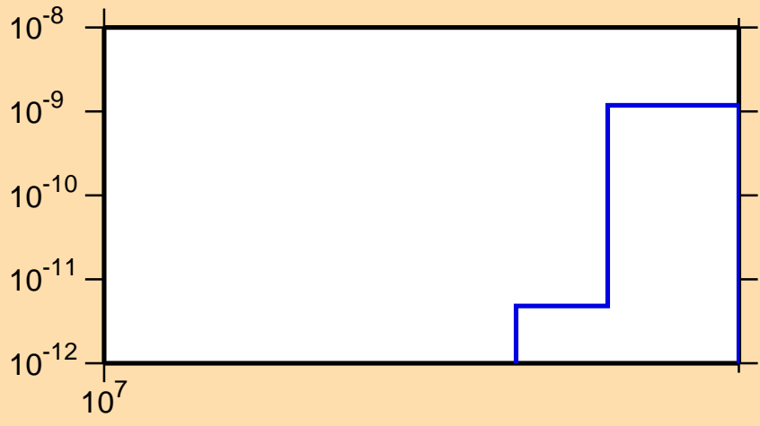
\sigma vs. E for ^{209}\text{Po}(n,\text{pt})
