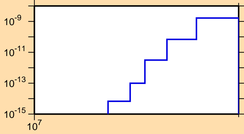
\sigma vs. E for ^{209}\text{Po} (mt 45)
