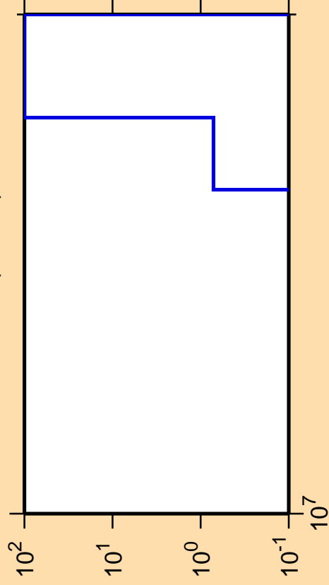
\Delta\sigma/\sigma vs. E for ^{209}\text{Po} (mt 34)
