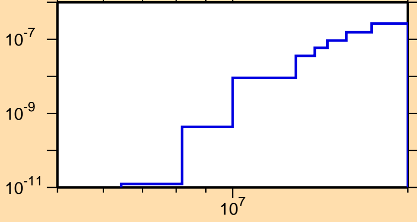
\sigma vs. E for ^{209}\text{Po}(n,p\alpha)
