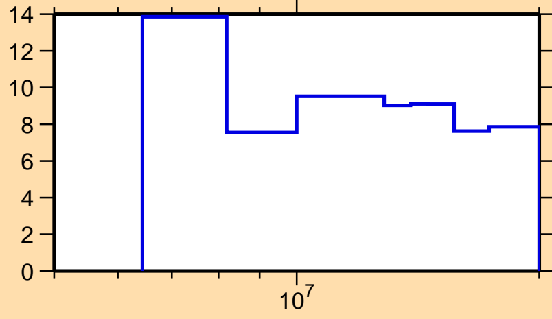
\Delta\sigma/\sigma vs. E for ^{209}\text{Po}(n,\text{el.})
