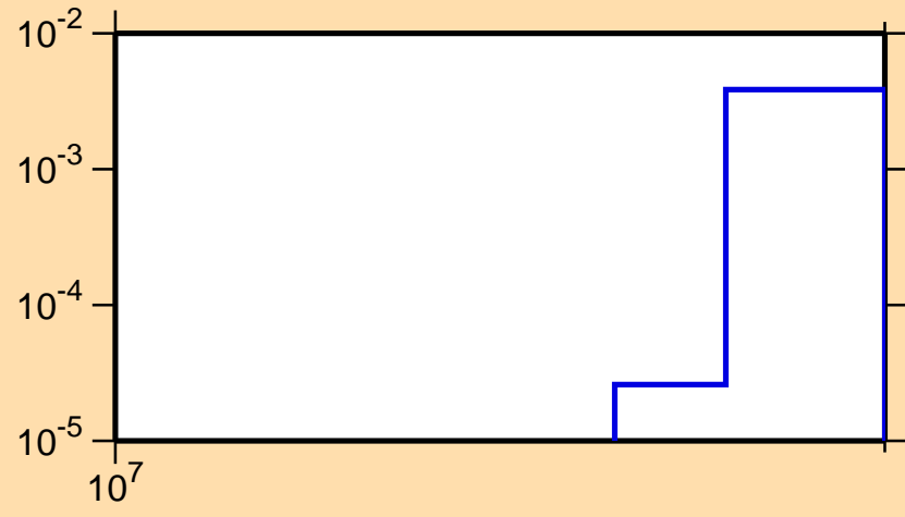
\sigma vs. E for ^{209}\text{Po}(n,3n\alpha)
