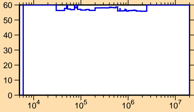
\Delta\sigma/\sigma vs. E for ^{209}\text{Po}(n,\gamma)
