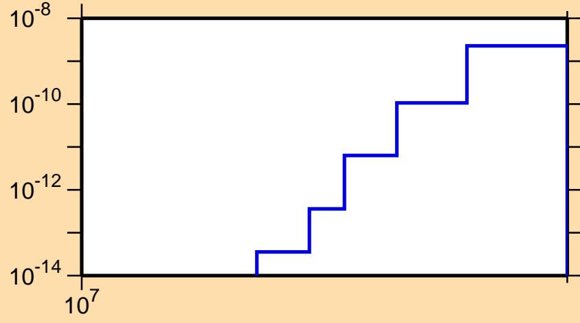
\sigma vs. E for ^{209}\text{Po}(\text{mt117})
