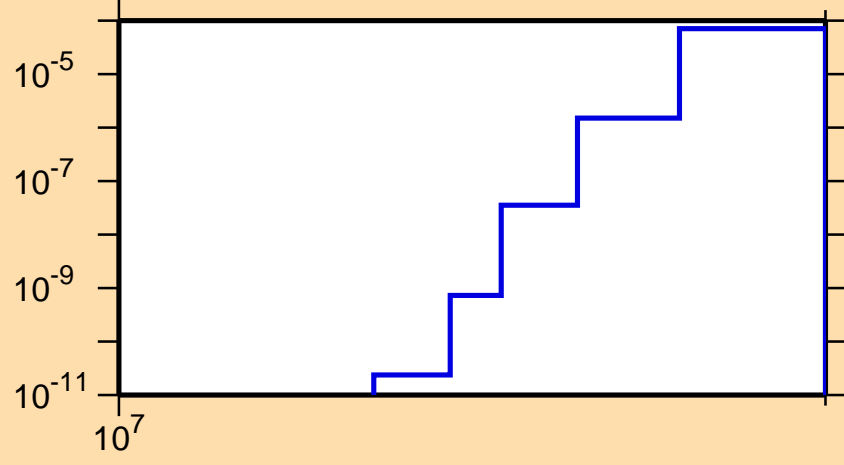
\sigma vs. E for ^{209}\text{Po}(n,\text{nd})
