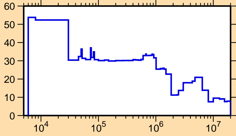
\Delta\sigma/\sigma vs. E for ^{209}\text{Po}(n,el.)
