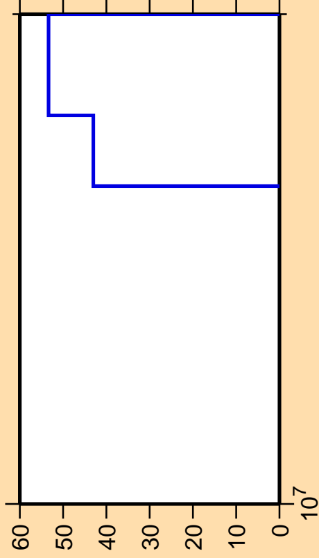
\Delta\sigma/\sigma vs. E for ^{209}\text{Po}(n,3n\alpha)
