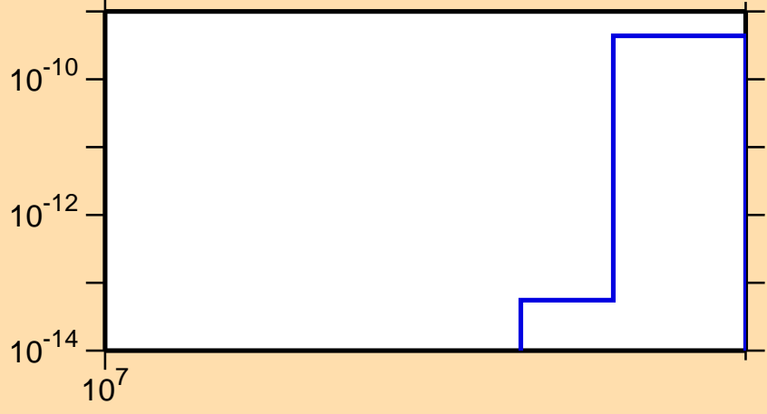
\sigma vs. E for ^{208}\text{Bi}(n,3n\alpha)
