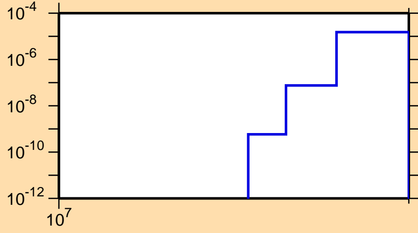
\sigma vs. E for ^{208}\text{Bi}(n,nt)
