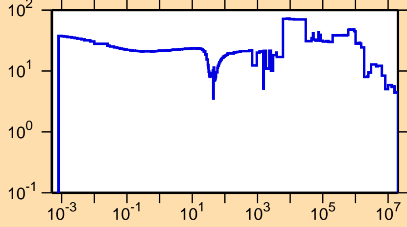
\Delta\sigma/\sigma vs. E for ^{208}\text{Bi}(n,\text{tot.})
