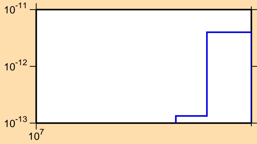
\sigma vs. E for ^{208}\text{Bi}(\text{mt117})
