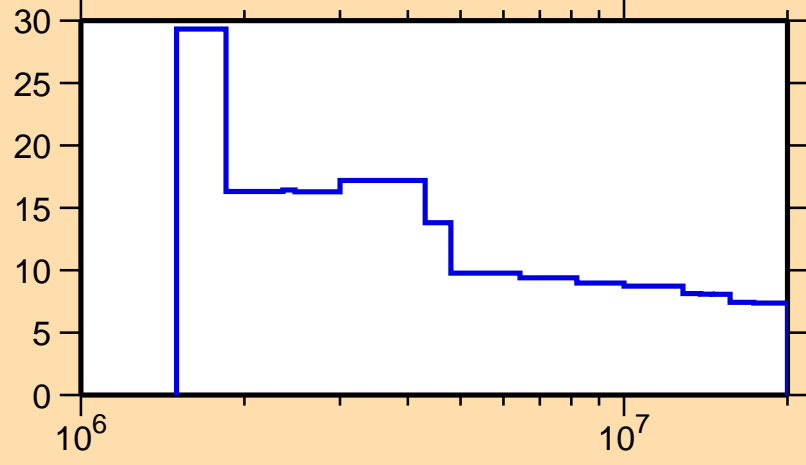
\Delta\sigma/\sigma vs. E for ^{208}\text{Bi}(n,n\text{onel.})
