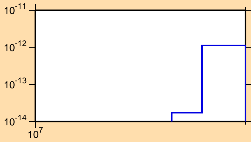
\sigma vs. E for ^{208}\text{Bi} (mt 45)
