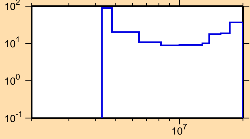
\Delta\sigma/\sigma vs. E for ^{210}\text{Bi}(n,2n)
