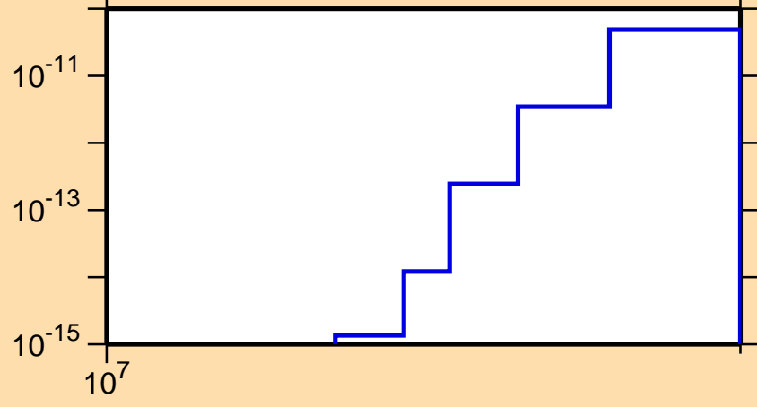
\sigma vs. E for ^{210}\text{Bi}(\text{mt117})
