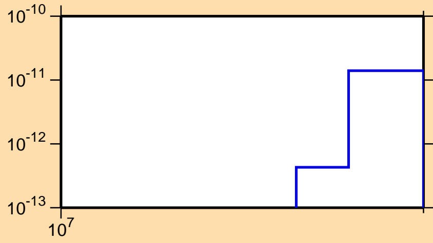
\sigma vs. E for ^{210}\text{Bi} (mt 45)
