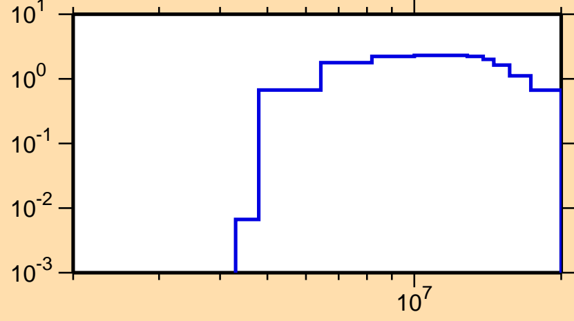
\sigma vs. E for ^{210}\text{Bi}(n,2n)
