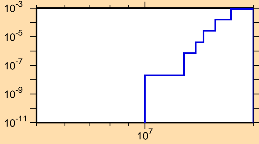
\sigma vs. E for ^{210}\text{Bi}(n,\text{nd})
