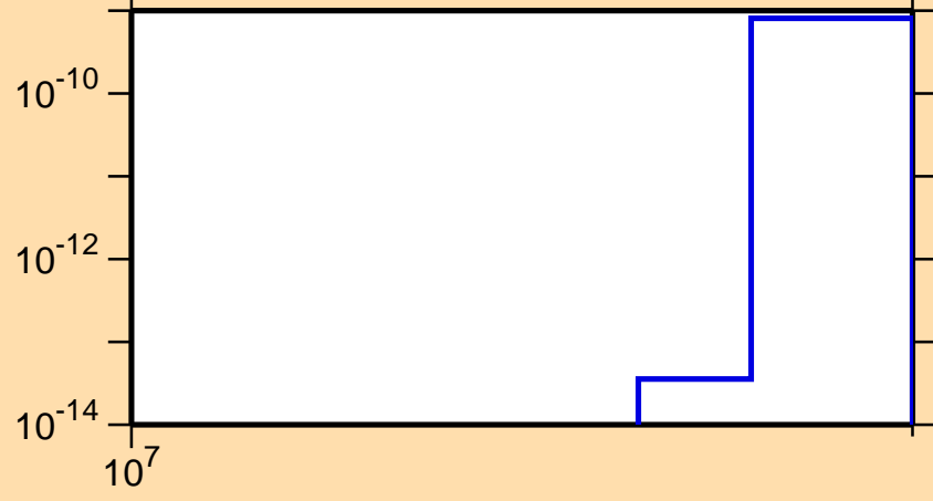
\sigma vs. E for ^{210}\text{Bi} (mt 11)
