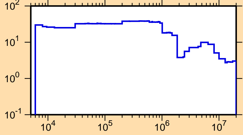
\Delta\sigma/\sigma vs. E for ^{204}\text{Tl}(n,\text{tot.})
