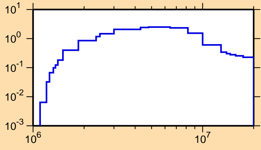
\sigma vs. E for ^{204}\text{Tl}(n,n\text{cont.})
