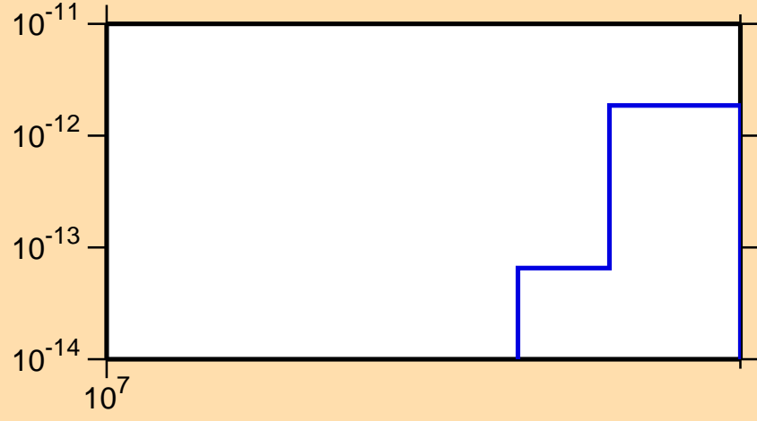
\sigma vs. E for ^{204}\text{Tl}(n,p\alpha)
