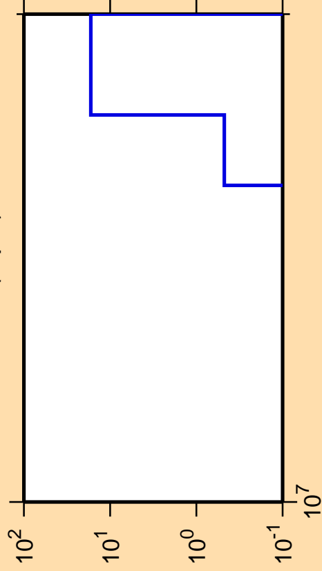
\Delta\sigma/\sigma vs. E for ^{204}\text{Tl}(n,p\alpha)
