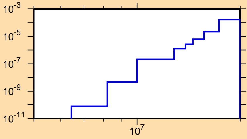
\sigma vs. E for ^{204}\text{Tl}(n,n\alpha)
