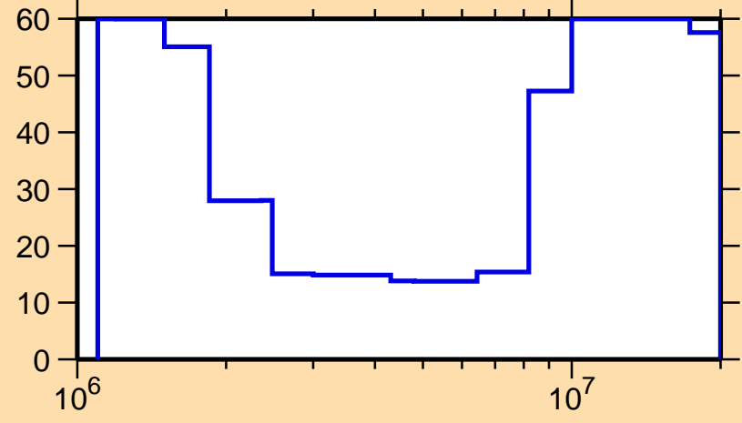
\Delta\sigma/\sigma vs. E for ^{204}\text{Tl}(n,ncont.)
