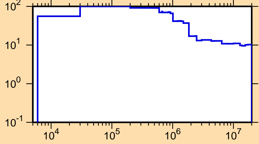
\Delta\sigma/\sigma vs. E for ^{204}\text{Tl}(n,\text{nonel.})
