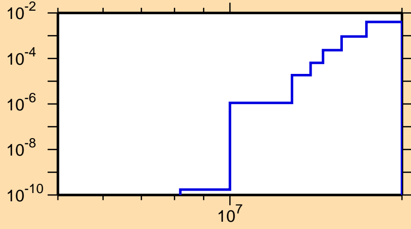
\sigma vs. E for ^{204}\text{Tl}(n,np)
