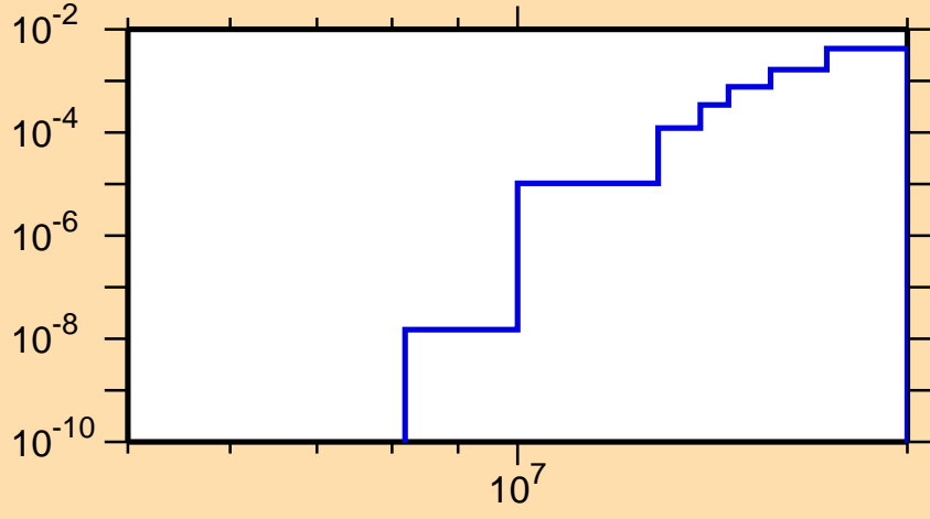
\sigma vs. E for ^{202}\text{Tl}(n,d)
