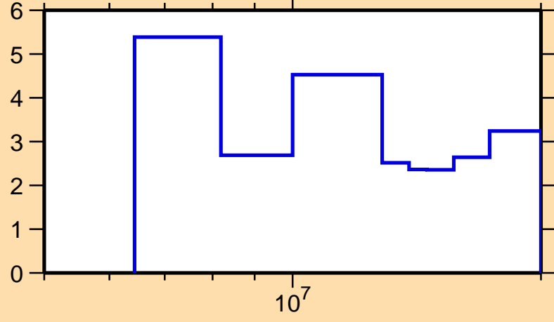
\Delta\sigma/\sigma vs. E for ^{202}\text{Tl}(n,\text{tot.})
