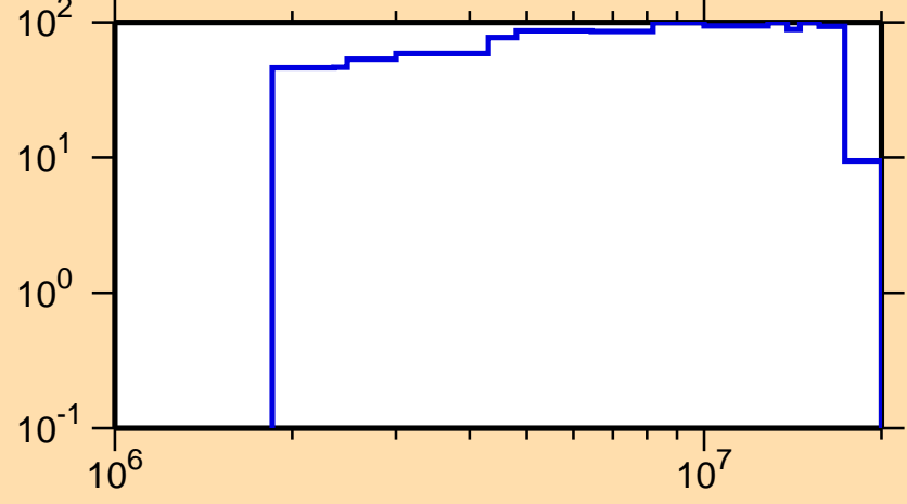
\Delta\sigma/\sigma vs. E for ^{202}\text{Tl}(n,n_1)
