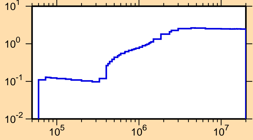
\sigma vs. E for ^{200}\text{Hg}(n,\text{nonel.})
