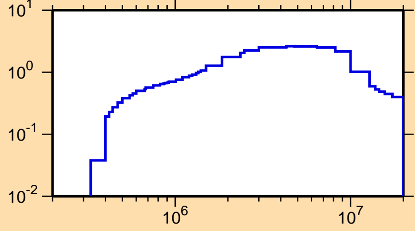
\sigma vs. E for ^{200}\text{Hg}(n,\text{inel.})
