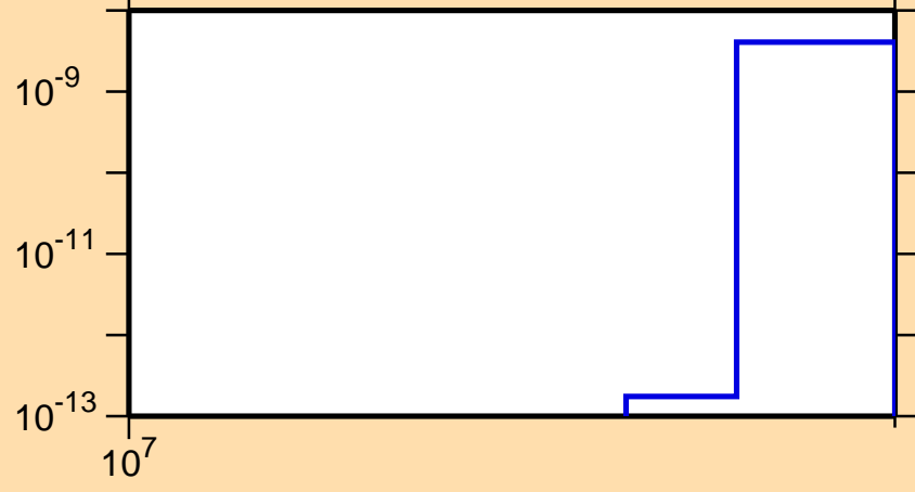
\sigma vs. E for ^{200}\text{Hg}(n,nt)
