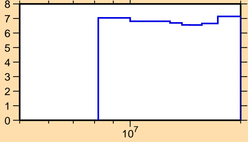
\Delta\sigma/\sigma vs. E for ^{194}\text{Pt}(n,\text{nonel.})
