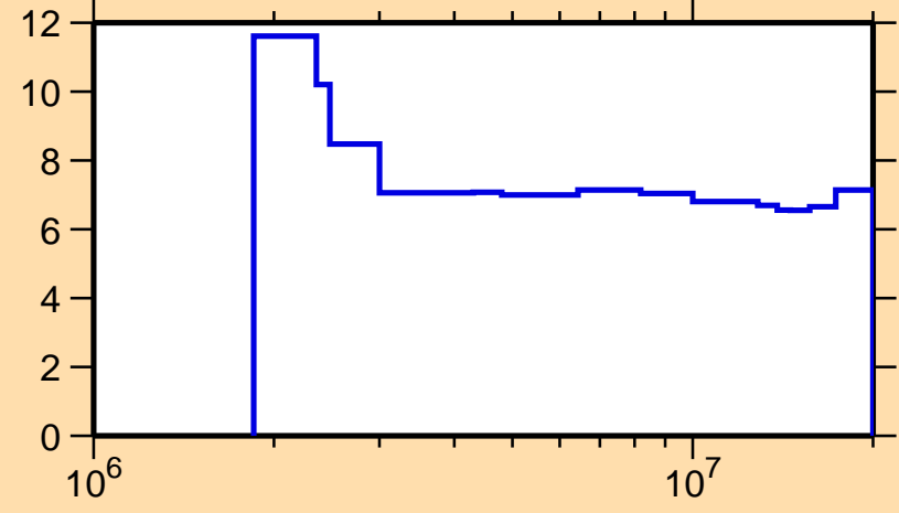
\Delta\sigma/\sigma vs. E for ^{194}\text{Pt}(n,n\text{onrel.})
