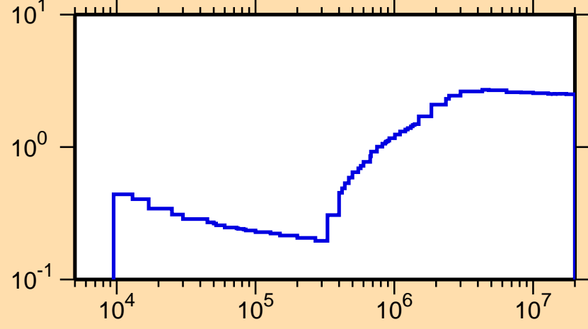
\sigma vs. E for ^{194}\text{Pt}(n,\text{nonel.})
