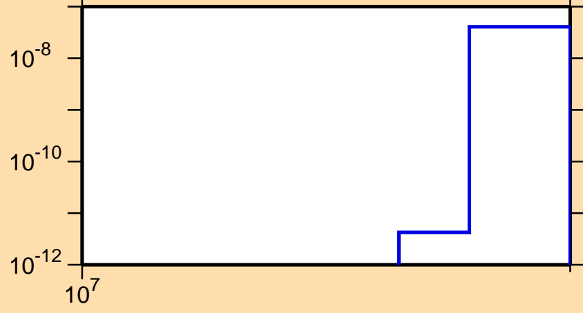
\sigma vs. E for ^{194}\text{Pt}(n,nt)
