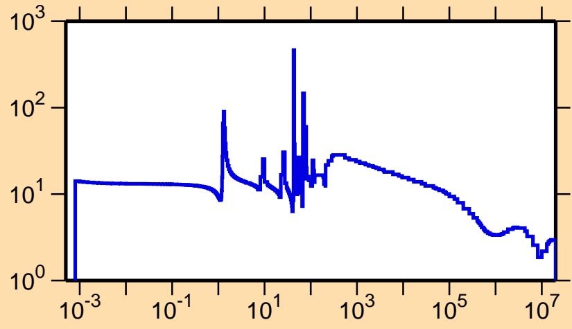
\sigma vs. E for ^{193}\text{Ir}(n,\text{el.})
