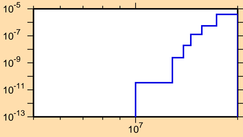
\sigma vs. E for ^{185}\text{Re}(n,2n\alpha)
