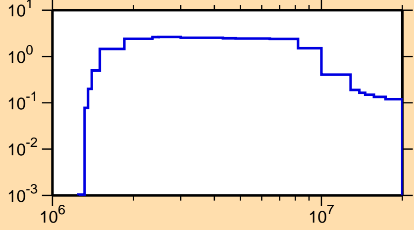
\sigma vs. E for ^{185}\text{Re}(n,n\text{cont.})
