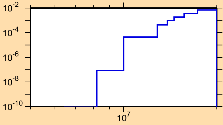
\sigma vs. E for ^{185}\text{Re}(n,d)
