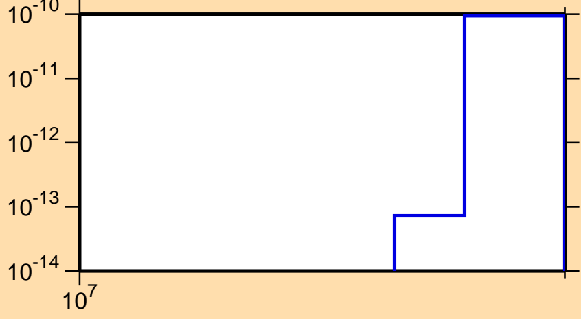
\sigma vs. E for ^{185}\text{Re}(n,3n\alpha)
