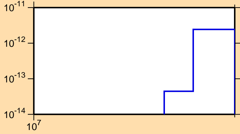
\sigma vs. E for ^{185}\text{Re} (mt 45)
